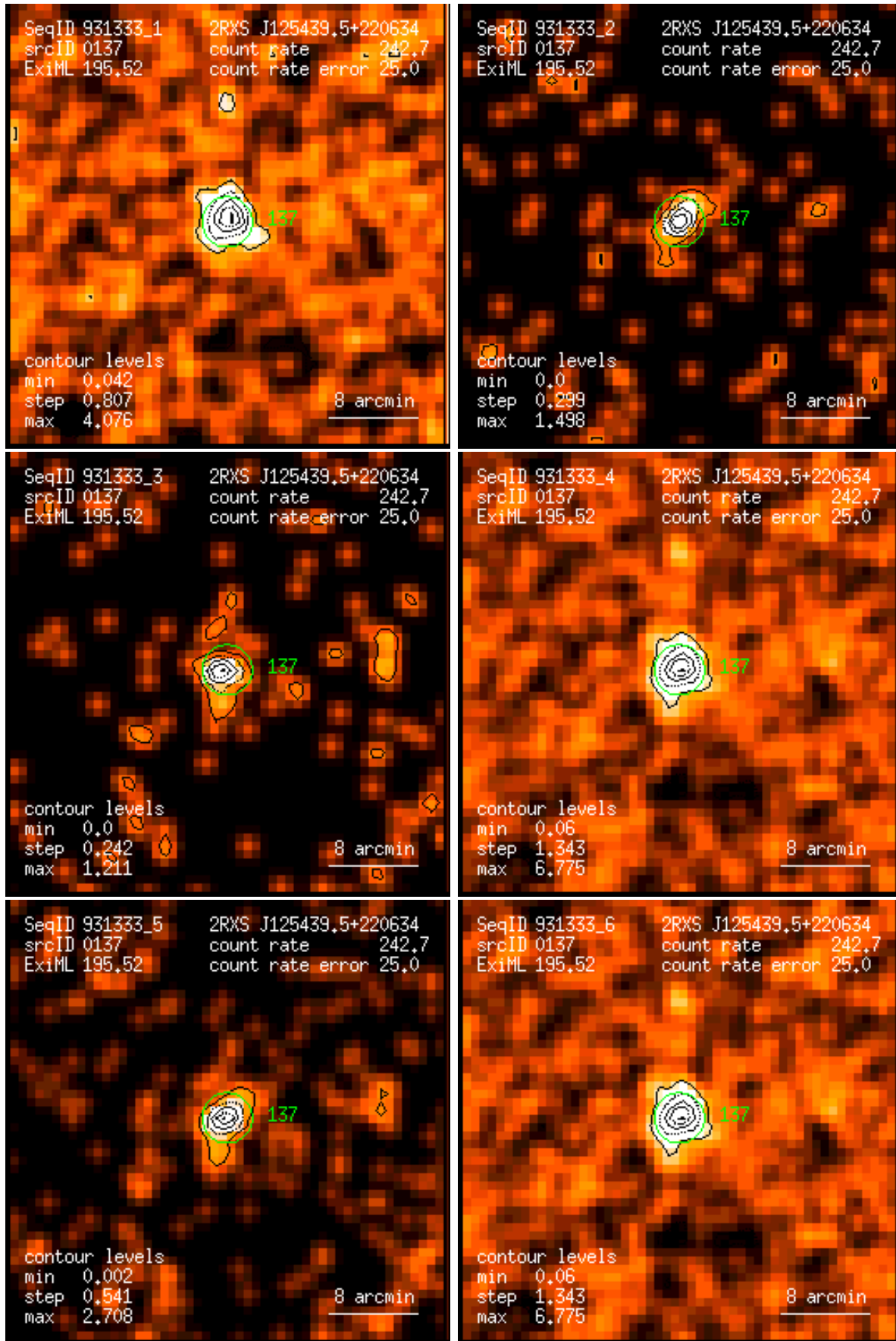
Figure 137: RASS 931333: detection 0137: band rate images, Gaussian filter: (1) PSPC channels 11 – 41, (2) 52 – 90, (3) 91 – 201, (4) 11 – 235, (5) 52 – 201, (6) 11 – 201. Broad band rates in counts/ks. Band rate contour levels in counts/ks/arcmin 2 .
