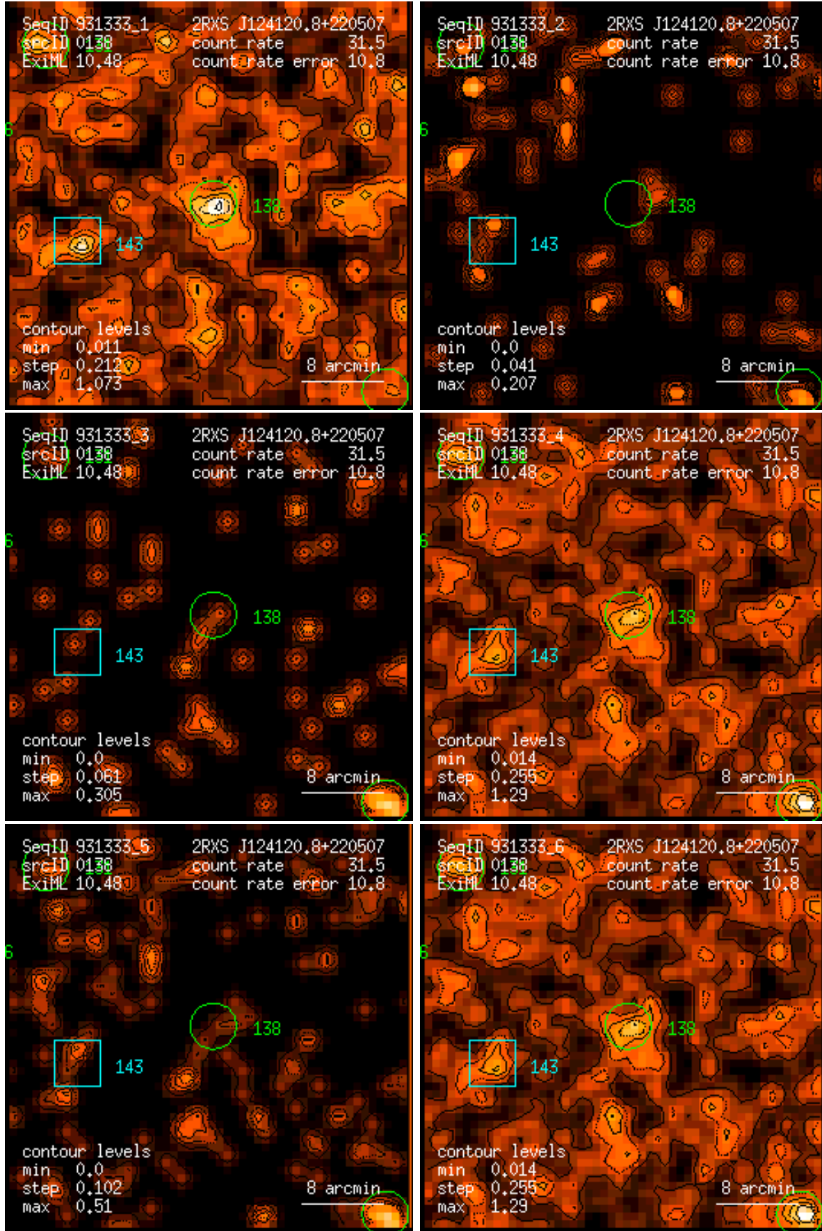
Figure 138: RASS 931333: detection 0138: band rate images, Gaussian filter: (1) PSPC channels 11 – 41, (2) 52 – 90, (3) 91 – 201, (4) 11 – 235, (5) 52 – 201, (6) 11 – 201. Broad band rates in counts/ks. Band rate contour levels in counts/ks/arcmin 2 .
