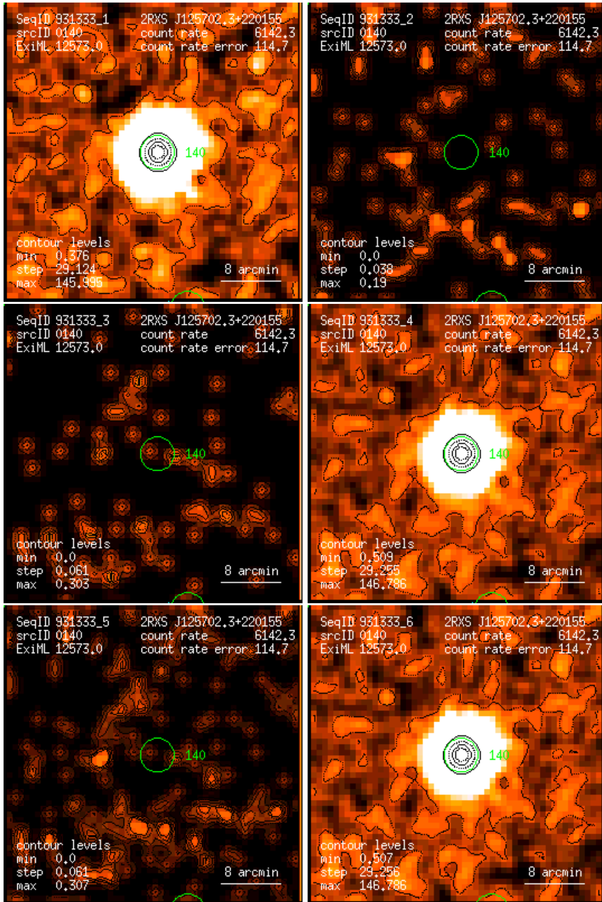
Figure 140: RASS 931333: detection 0140: band rate images, Gaussian filter: (1) PSPC channels 11 – 41, (2) 52 – 90, (3) 91 – 201, (4) 11 – 235, (5) 52 – 201, (6) 11 – 201. Broad band rates in counts/ks. Band rate contour levels in counts/ks/arcmin 2 .
