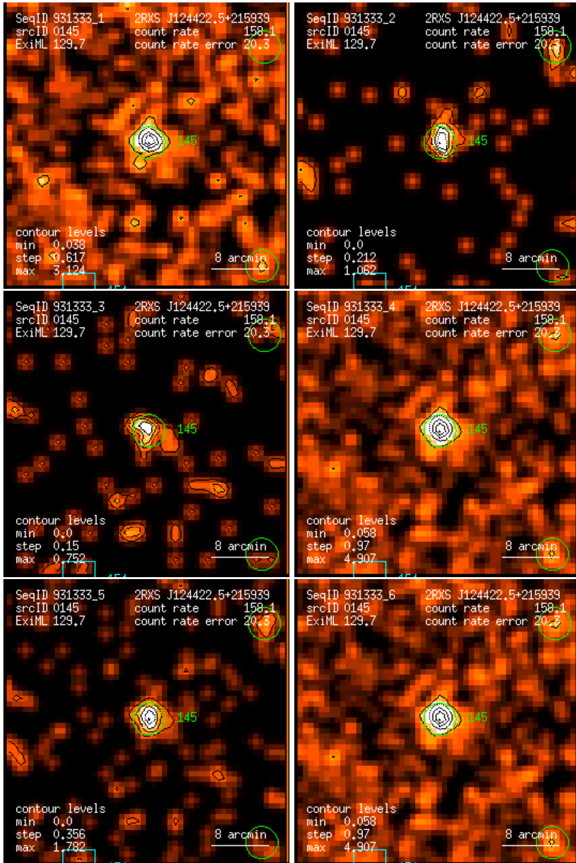
Figure 145: RASS 931333: detection 0145: band rate images, Gaussian filter: (1) PSPC channels 11 – 41, (2) 52 – 90, (3) 91 – 201, (4) 11 – 235, (5) 52 – 201, (6) 11 – 201. Broad band rates in counts/ks. Band rate contour levels in counts/ks/arcmin 2 .
