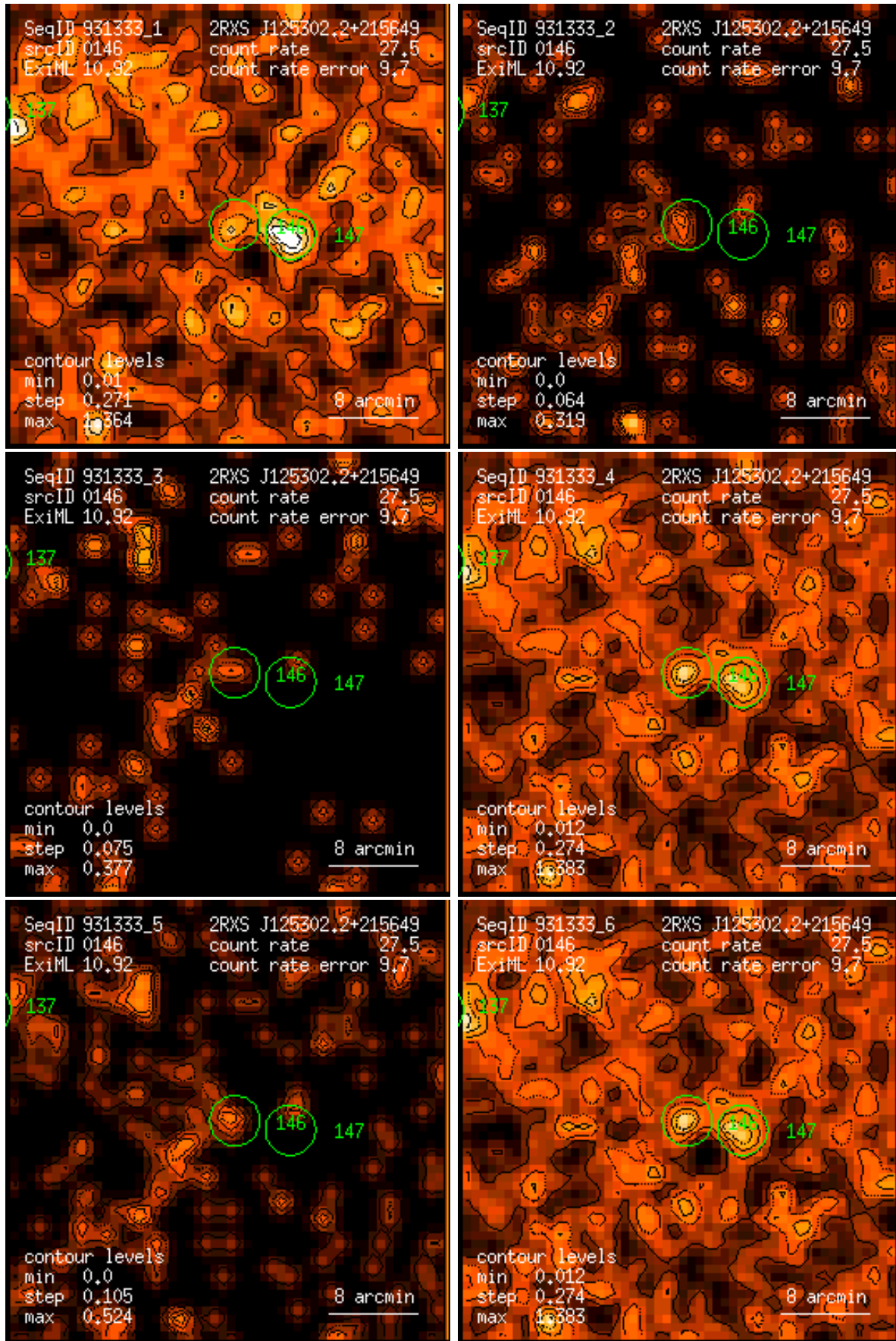
Figure 146: RASS 931333: detection 0146: band rate images, Gaussian filter: (1) PSPC channels 11 – 41, (2) 52 – 90, (3) 91 – 201, (4) 11 – 235, (5) 52 – 201, (6) 11 – 201. Broad band rates in counts/ks. Band rate contour levels in counts/ks/arcmin 2 .
