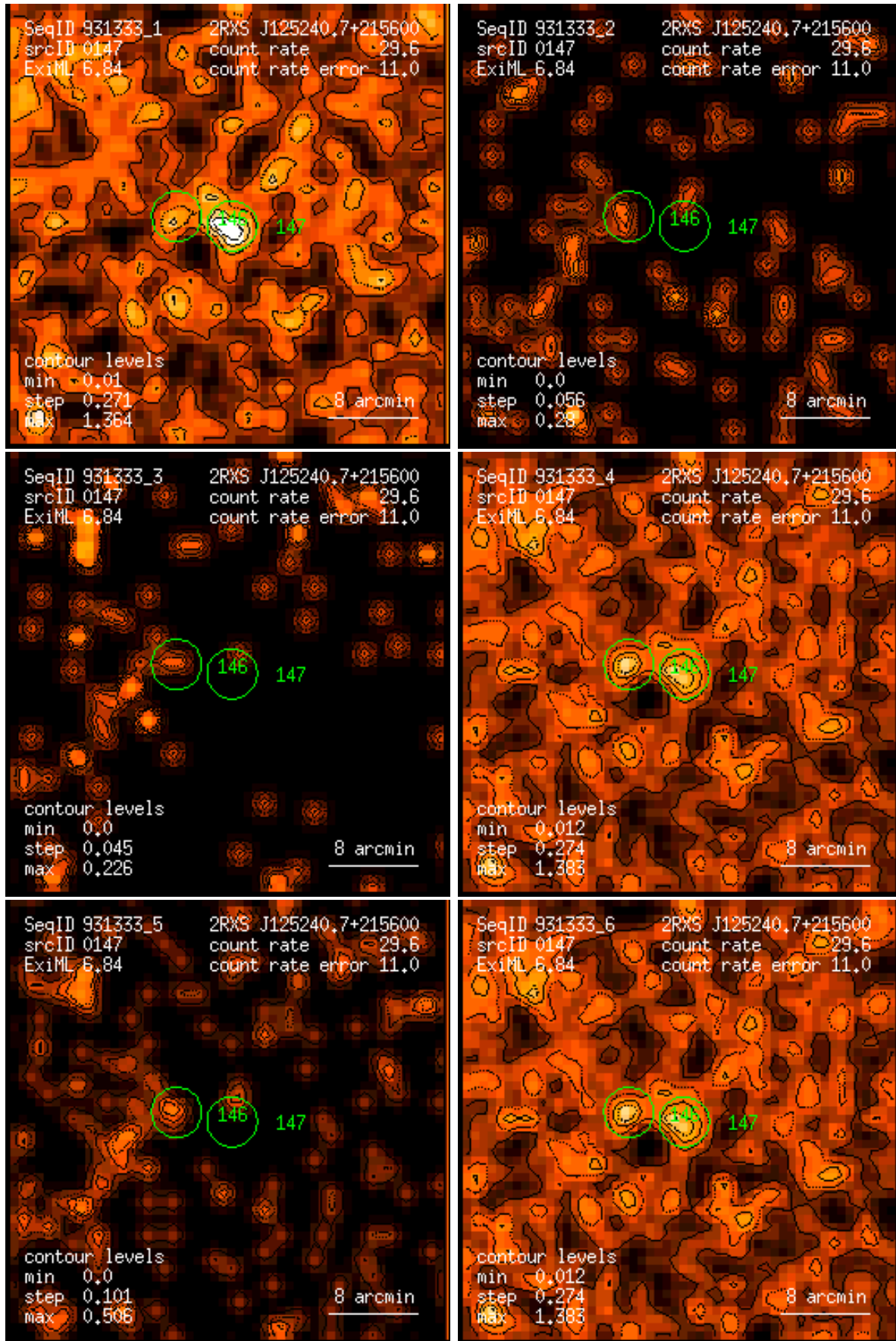
Figure 147: RASS 931333: detection 0147: band rate images, Gaussian filter: (1) PSPC channels 11 – 41, (2) 52 – 90, (3) 91 – 201, (4) 11 – 235, (5) 52 – 201, (6) 11 – 201. Broad band rates in counts/ks. Band rate contour levels in counts/ks/arcmin 2 .
