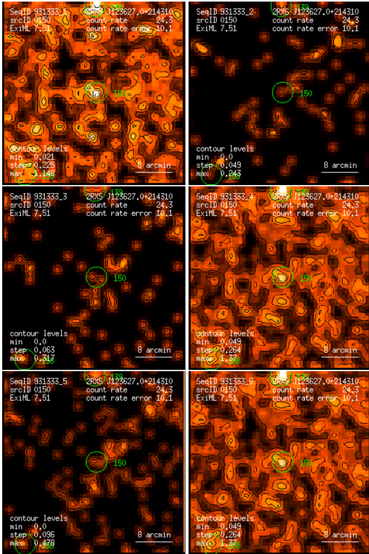
Figure 150: RASS 931333: detection 0150: band rate images, Gaussian filter: (1) PSPC channels 11 – 41, (2) 52 – 90, (3) 91 – 201, (4) 11 – 235, (5) 52 – 201, (6) 11 – 201. Broad band rates in counts/ks. Band rate contour levels in counts/ks/arcmin 2 .
