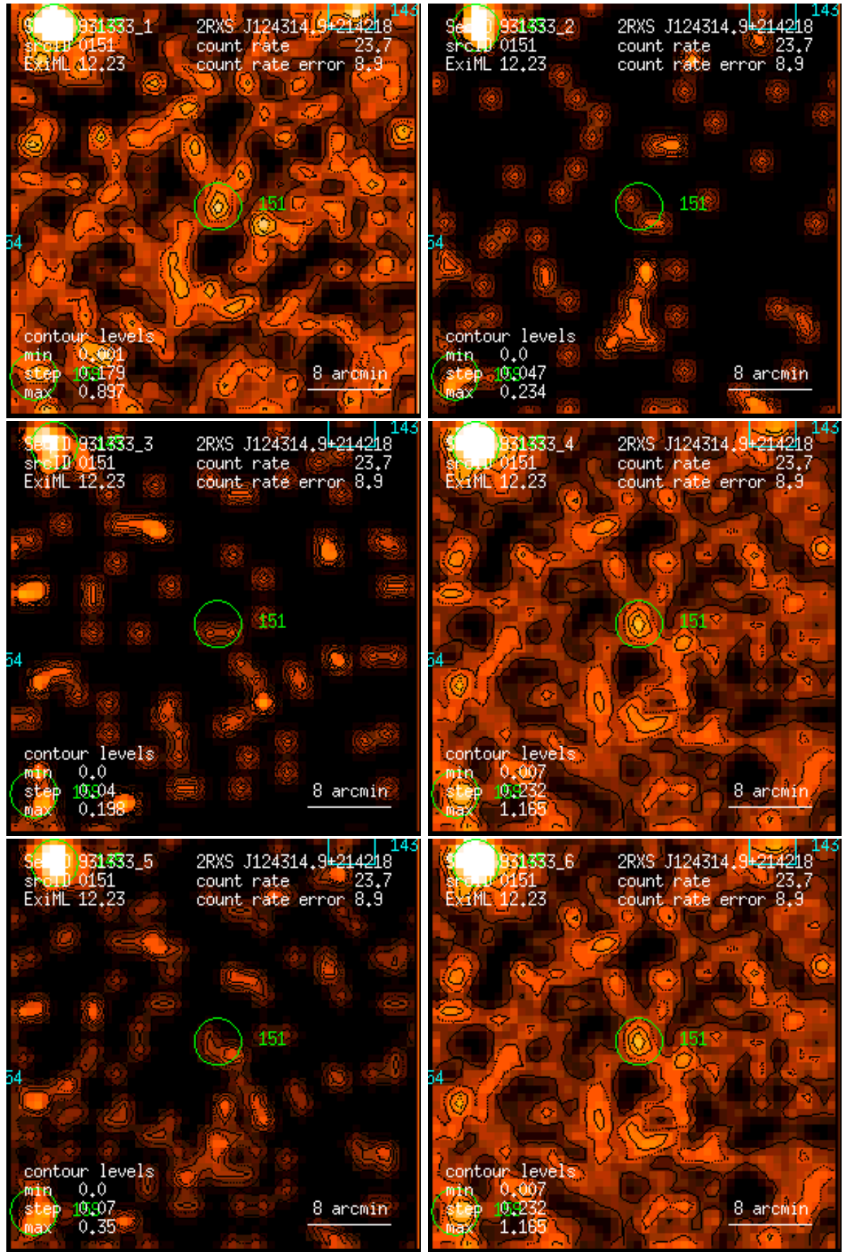
Figure 151: RASS 931333: detection 0151: band rate images, Gaussian filter: (1) PSPC channels 11 – 41, (2) 52 – 90, (3) 91 – 201, (4) 11 – 235, (5) 52 – 201, (6) 11 – 201. Broad band rates in counts/ks. Band rate contour levels in counts/ks/arcmin 2 .
