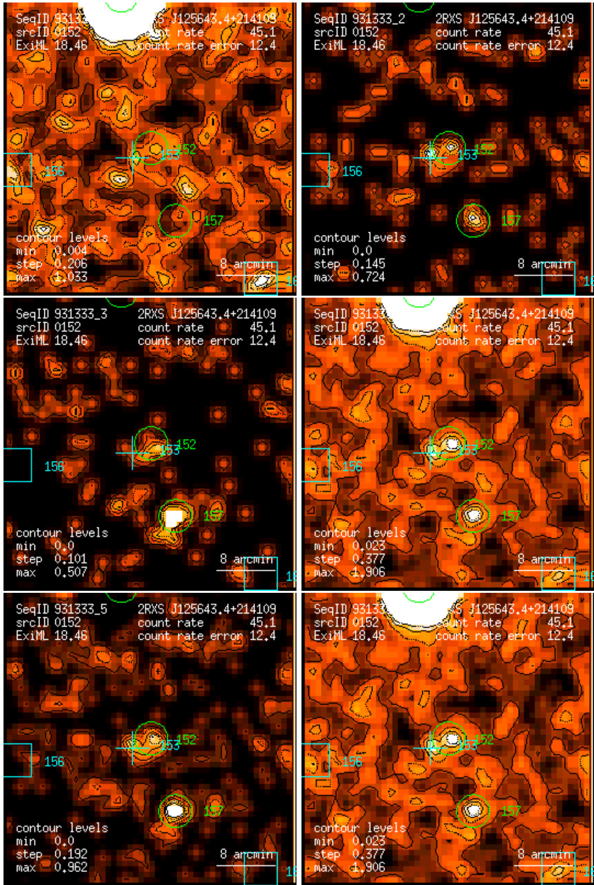
Figure 152: RASS 931333: detection 0152: band rate images, Gaussian filter: (1) PSPC channels 11 – 41, (2) 52 – 90, (3) 91 – 201, (4) 11 – 235, (5) 52 – 201, (6) 11 – 201. Broad band rates in counts/ks. Band rate contour levels in counts/ks/arcmin 2 .
