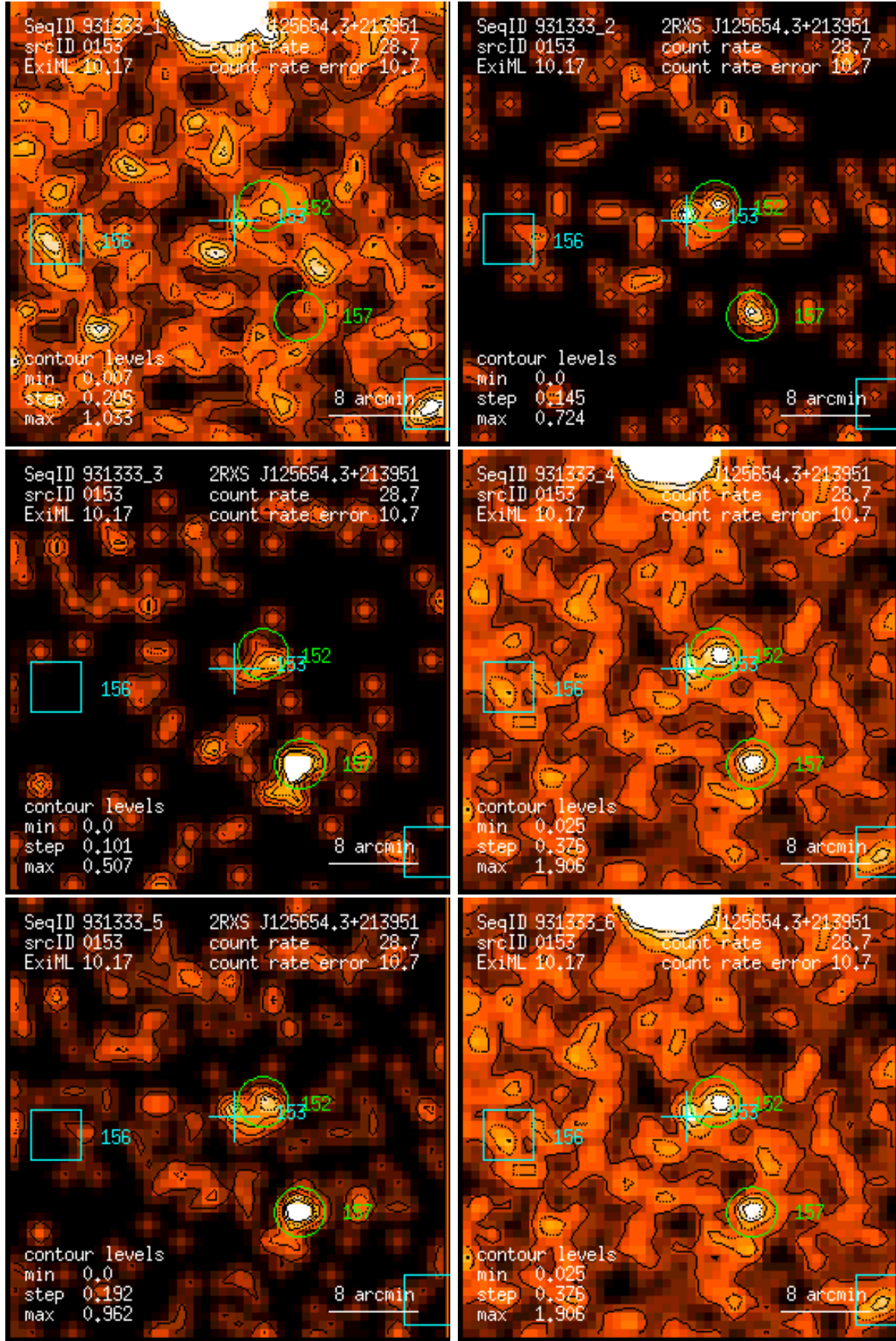
Figure 153: RASS 931333: detection 0153: band rate images, Gaussian filter: (1) PSPC channels 11 – 41, (2) 52 – 90, (3) 91 – 201, (4) 11 – 235, (5) 52 – 201, (6) 11 – 201. Broad band rates in counts/ks. Band rate contour levels in counts/ks/arcmin 2 .
