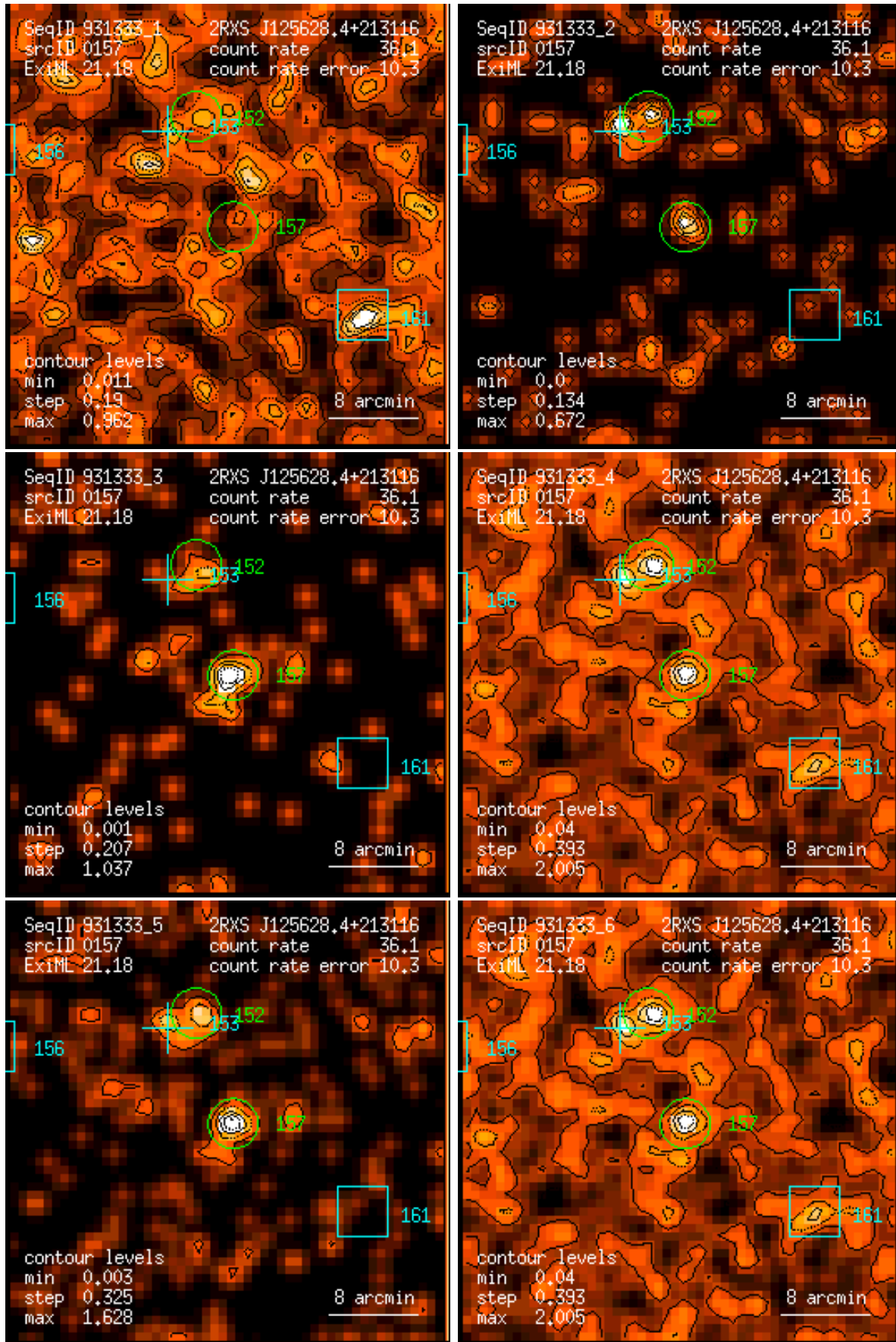
Figure 157: RASS 931333: detection 0157: band rate images, Gaussian filter: (1) PSPC channels 11 – 41, (2) 52 – 90, (3) 91 – 201, (4) 11 – 235, (5) 52 – 201, (6) 11 – 201. Broad band rates in counts/ks. Band rate contour levels in counts/ks/arcmin 2 .
