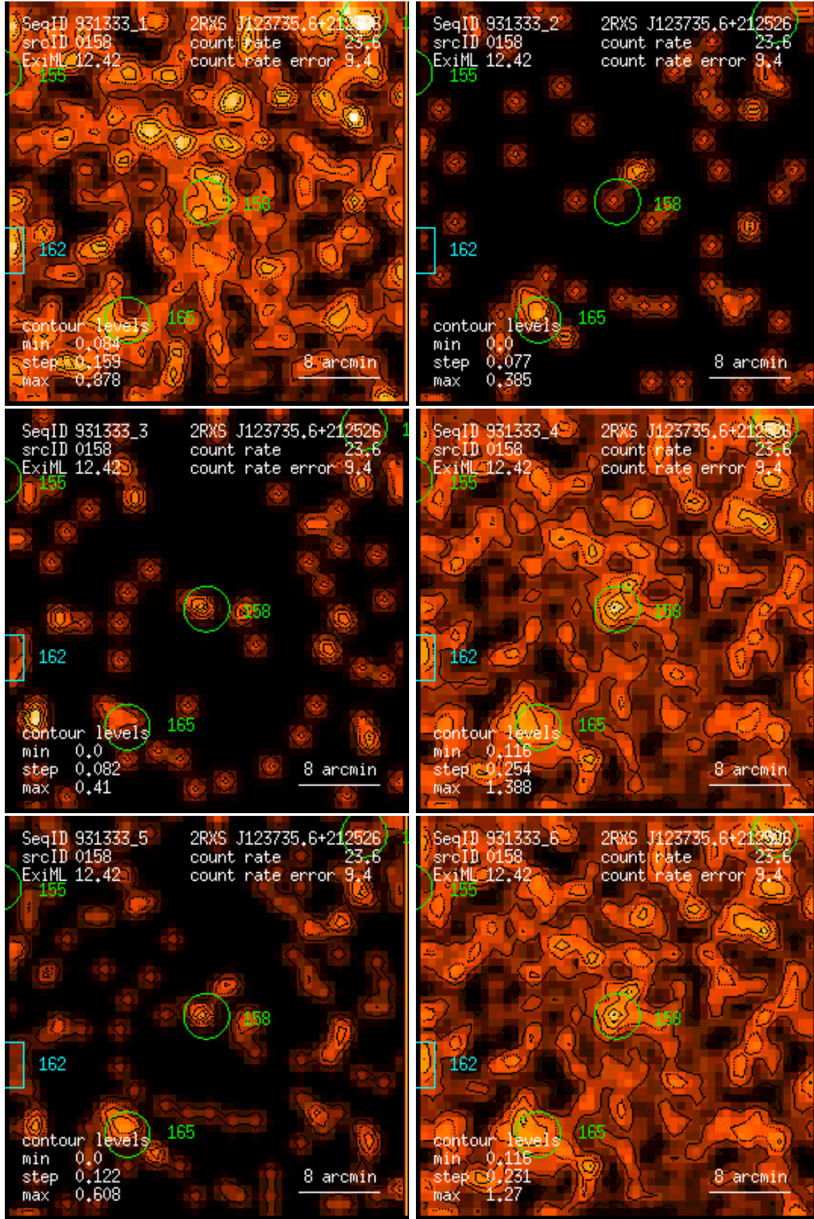
Figure 158: RASS 931333: detection 0158: band rate images, Gaussian filter: (1) PSPC channels 11 – 41, (2) 52 – 90, (3) 91 – 201, (4) 11 – 235, (5) 52 – 201, (6) 11 – 201. Broad band rates in counts/ks. Band rate contour levels in counts/ks/arcmin 2 .
