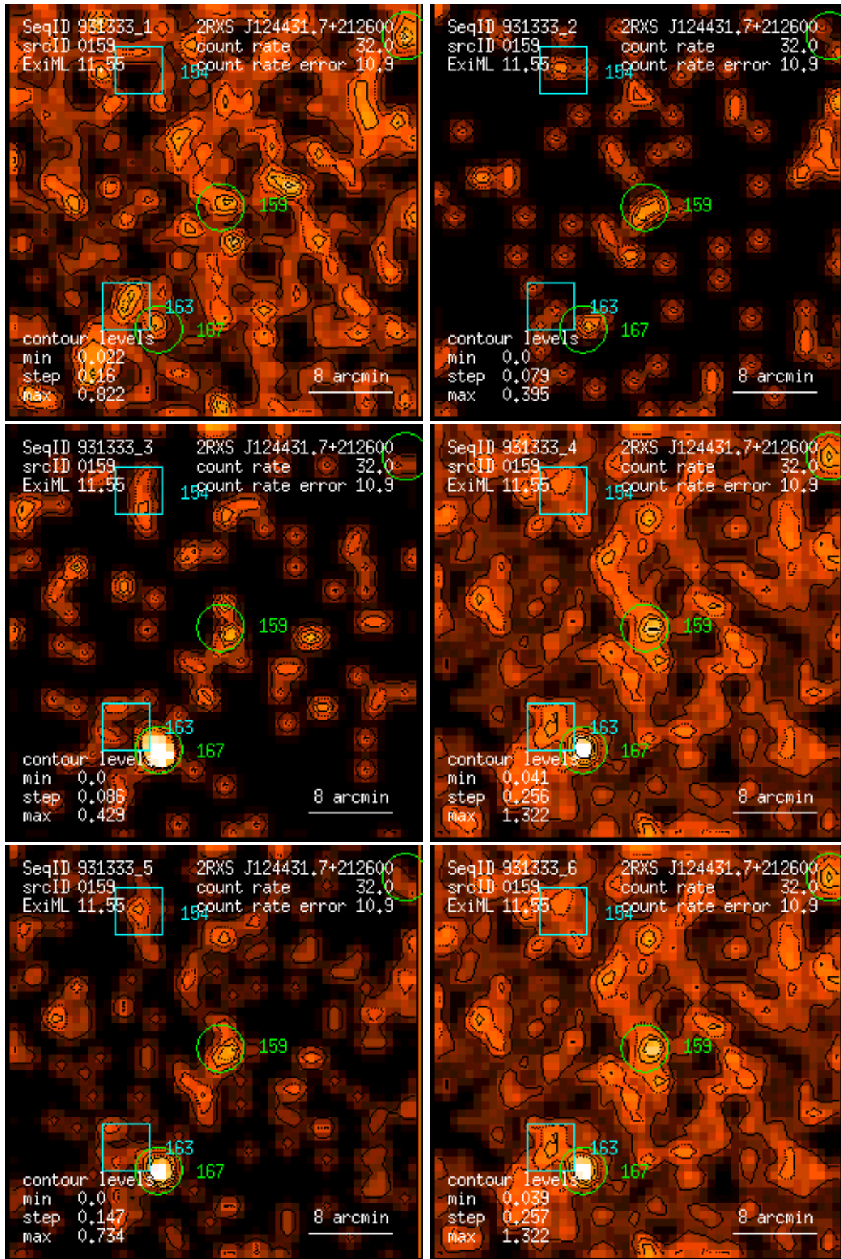
Figure 159: RASS 931333: detection 0159: band rate images, Gaussian filter: (1) PSPC channels 11 – 41, (2) 52 – 90, (3) 91 – 201, (4) 11 – 235, (5) 52 – 201, (6) 11 – 201. Broad band rates in counts/ks. Band rate contour levels in counts/ks/arcmin 2 .
