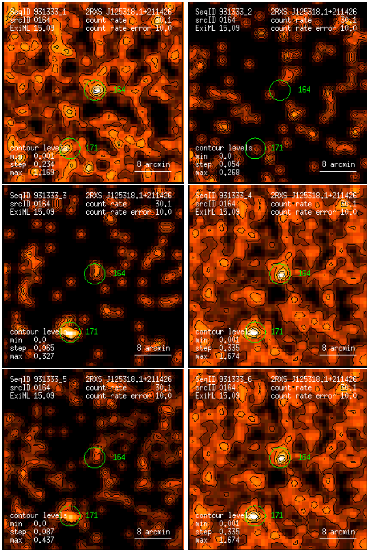
Figure 164: RASS 931333: detection 0164: band rate images, Gaussian filter: (1) PSPC channels 11 – 41, (2) 52 – 90, (3) 91 – 201, (4) 11 – 235, (5) 52 – 201, (6) 11 – 201. Broad band rates in counts/ks. Band rate contour levels in counts/ks/arcmin 2 .
