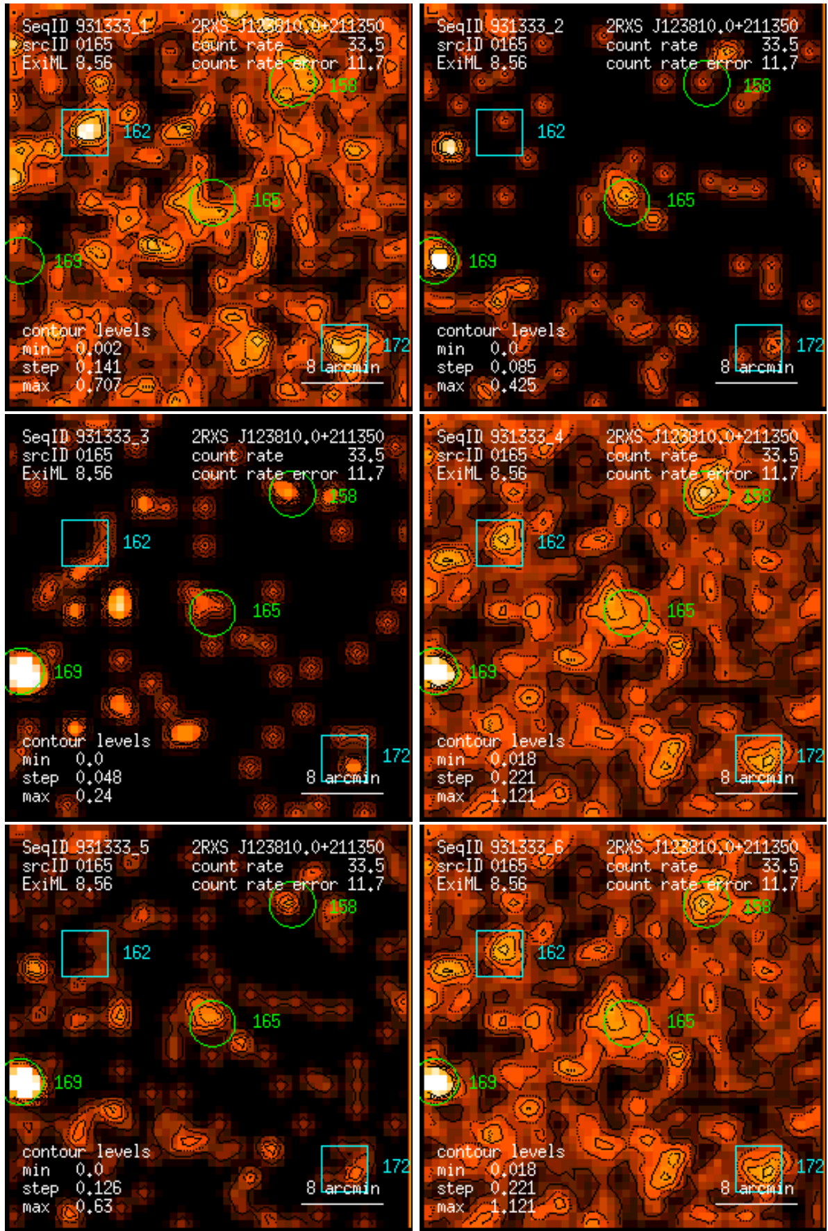
Figure 165: RASS 931333: detection 0165: band rate images, Gaussian filter: (1) PSPC channels 11 – 41, (2) 52 – 90, (3) 91 – 201, (4) 11 – 235, (5) 52 – 201, (6) 11 – 201. Broad band rates in counts/ks. Band rate contour levels in counts/ks/arcmin 2 .
