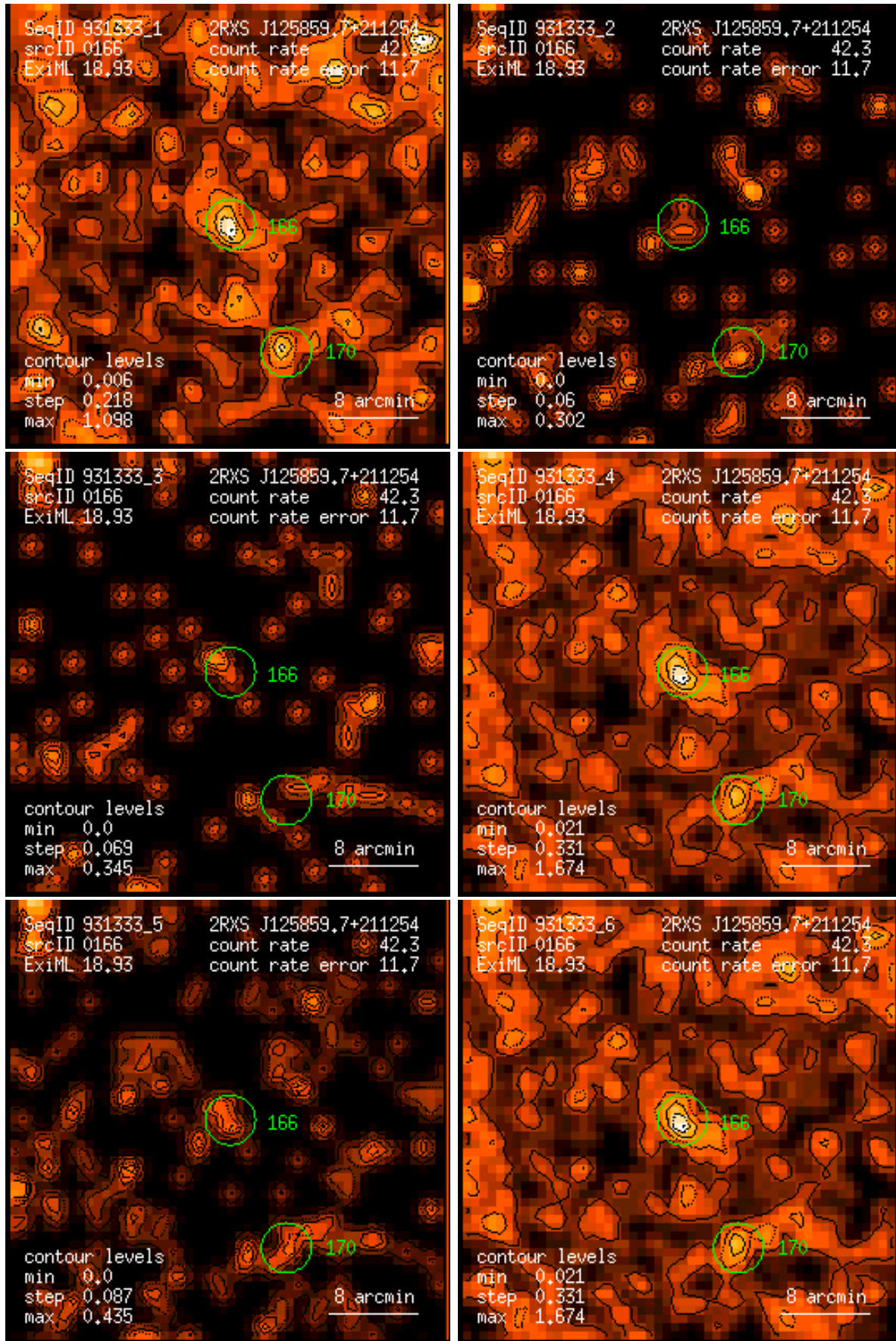
Figure 166: RASS 931333: detection 0166: band rate images, Gaussian filter: (1) PSPC channels 11 – 41, (2) 52 – 90, (3) 91 – 201, (4) 11 – 235, (5) 52 – 201, (6) 11 – 201. Broad band rates in counts/ks. Band rate contour levels in counts/ks/arcmin 2 .
