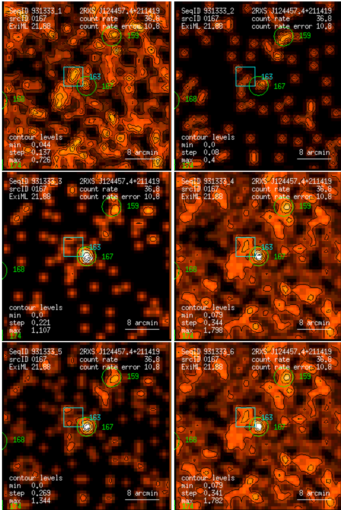
Figure 167: RASS 931333: detection 0167: band rate images, Gaussian filter: (1) PSPC channels 11 – 41, (2) 52 – 90, (3) 91 – 201, (4) 11 – 235, (5) 52 – 201, (6) 11 – 201. Broad band rates in counts/ks. Band rate contour levels in counts/ks/arcmin 2 .
