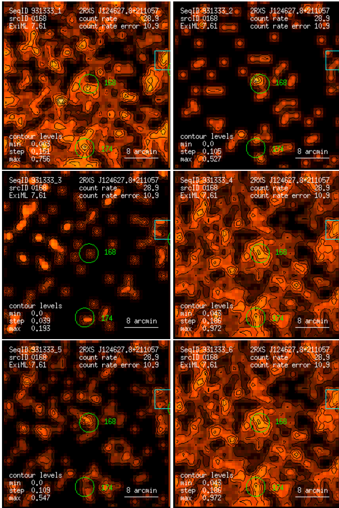
Figure 168: RASS 931333: detection 0168: band rate images, Gaussian filter: (1) PSPC channels 11 – 41, (2) 52 – 90, (3) 91 – 201, (4) 11 – 235, (5) 52 – 201, (6) 11 – 201. Broad band rates in counts/ks. Band rate contour levels in counts/ks/arcmin 2 .
