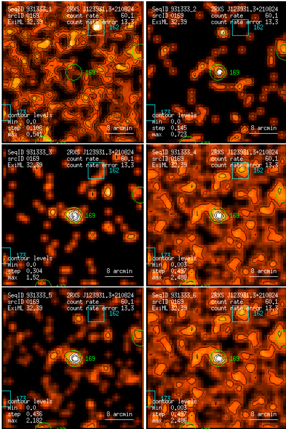
Figure 169: RASS 931333: detection 0169: band rate images, Gaussian filter: (1) PSPC channels 11 – 41, (2) 52 – 90, (3) 91 – 201, (4) 11 – 235, (5) 52 – 201, (6) 11 – 201. Broad band rates in counts/ks. Band rate contour levels in counts/ks/arcmin 2 .
