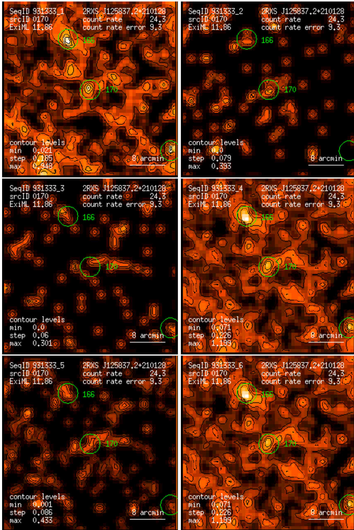
Figure 170: RASS 931333: detection 0170: band rate images, Gaussian filter: (1) PSPC channels 11 – 41, (2) 52 – 90, (3) 91 – 201, (4) 11 – 235, (5) 52 – 201, (6) 11 – 201. Broad band rates in counts/ks. Band rate contour levels in counts/ks/arcmin 2 .
