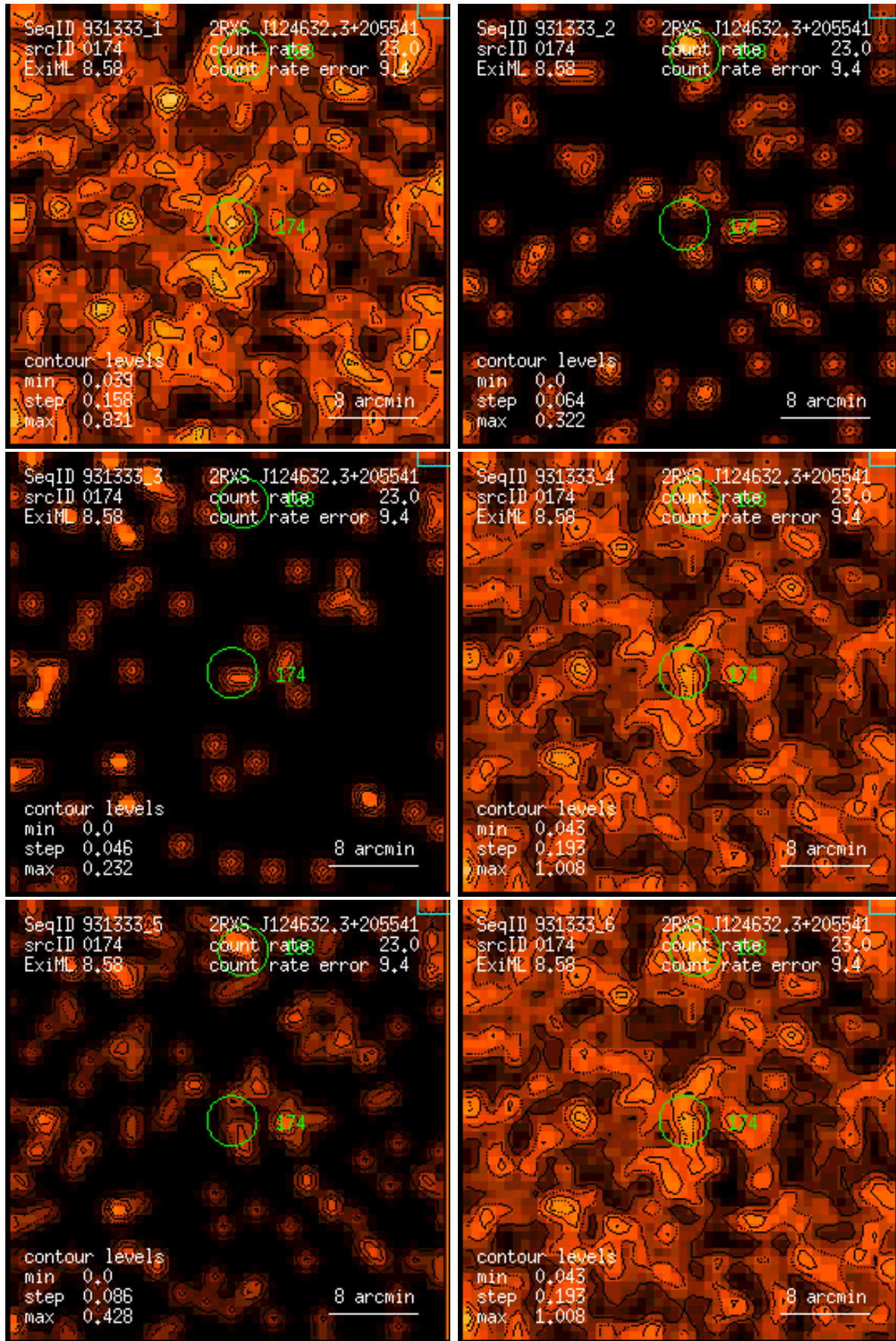
Figure 174: RASS 931333: detection 0174: band rate images, Gaussian filter: (1) PSPC channels 11 – 41, (2) 52 – 90, (3) 91 – 201, (4) 11 – 235, (5) 52 – 201, (6) 11 – 201. Broad band rates in counts/ks. Band rate contour levels in counts/ks/arcmin 2 .
