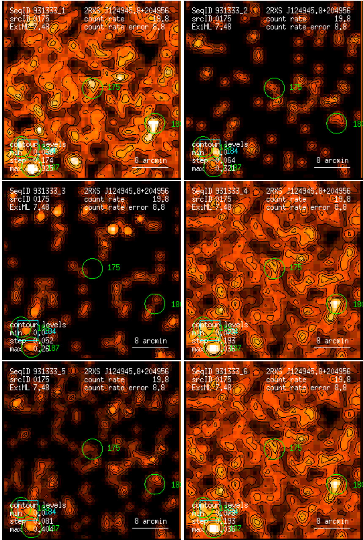
Figure 175: RASS 931333: detection 0175: band rate images, Gaussian filter: (1) PSPC channels 11 – 41, (2) 52 – 90, (3) 91 – 201, (4) 11 – 235, (5) 52 – 201, (6) 11 – 201. Broad band rates in counts/ks. Band rate contour levels in counts/ks/arcmin 2 .
