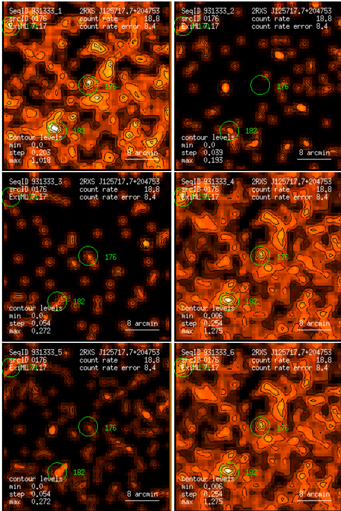
Figure 176: RASS 931333: detection 0176: band rate images, Gaussian filter: (1) PSPC channels 11 – 41, (2) 52 – 90, (3) 91 – 201, (4) 11 – 235, (5) 52 – 201, (6) 11 – 201. Broad band rates in counts/ks. Band rate contour levels in counts/ks/arcmin 2 .
