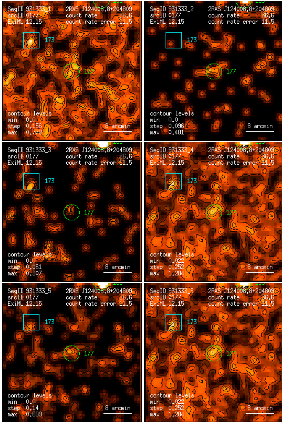
Figure 177: RASS 931333: detection 0177: band rate images, Gaussian filter: (1) PSPC channels 11 – 41, (2) 52 – 90, (3) 91 – 201, (4) 11 – 235, (5) 52 – 201, (6) 11 – 201. Broad band rates in counts/ks. Band rate contour levels in counts/ks/arcmin 2 .
