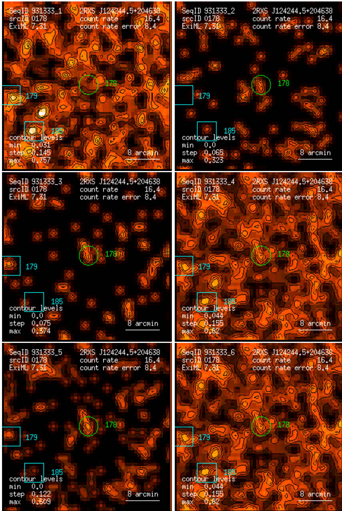
Figure 178: RASS 931333: detection 0178: band rate images, Gaussian filter: (1) PSPC channels 11 – 41, (2) 52 – 90, (3) 91 – 201, (4) 11 – 235, (5) 52 – 201, (6) 11 – 201. Broad band rates in counts/ks. Band rate contour levels in counts/ks/arcmin 2 .
