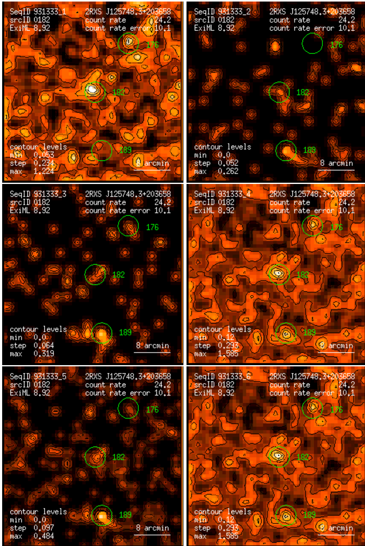
Figure 182: RASS 931333: detection 0182: band rate images, Gaussian filter: (1) PSPC channels 11 – 41, (2) 52 – 90, (3) 91 – 201, (4) 11 – 235, (5) 52 – 201, (6) 11 – 201. Broad band rates in counts/ks. Band rate contour levels in counts/ks/arcmin 2 .
