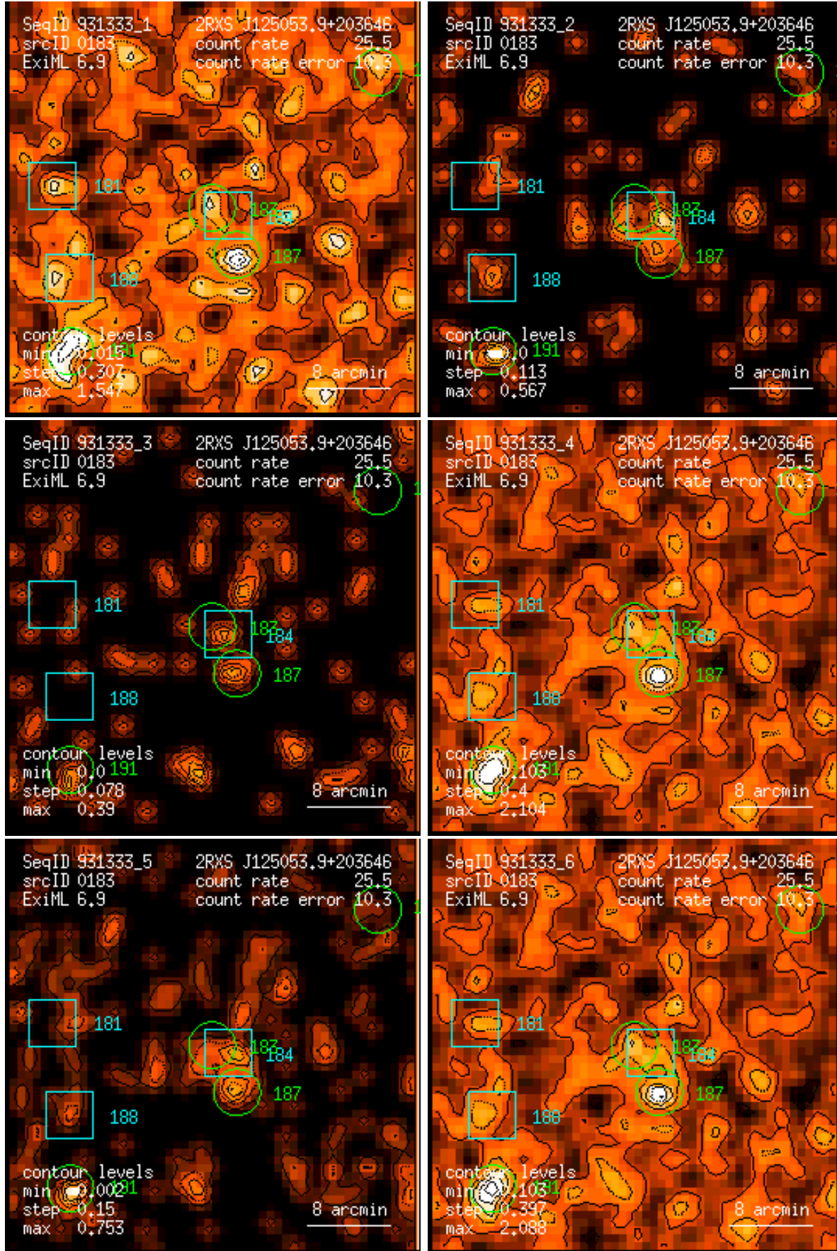
Figure 183: RASS 931333: detection 0183: band rate images, Gaussian filter: (1) PSPC channels 11 – 41, (2) 52 – 90, (3) 91 – 201, (4) 11 – 235, (5) 52 – 201, (6) 11 – 201. Broad band rates in counts/ks. Band rate contour levels in counts/ks/arcmin 2 .
