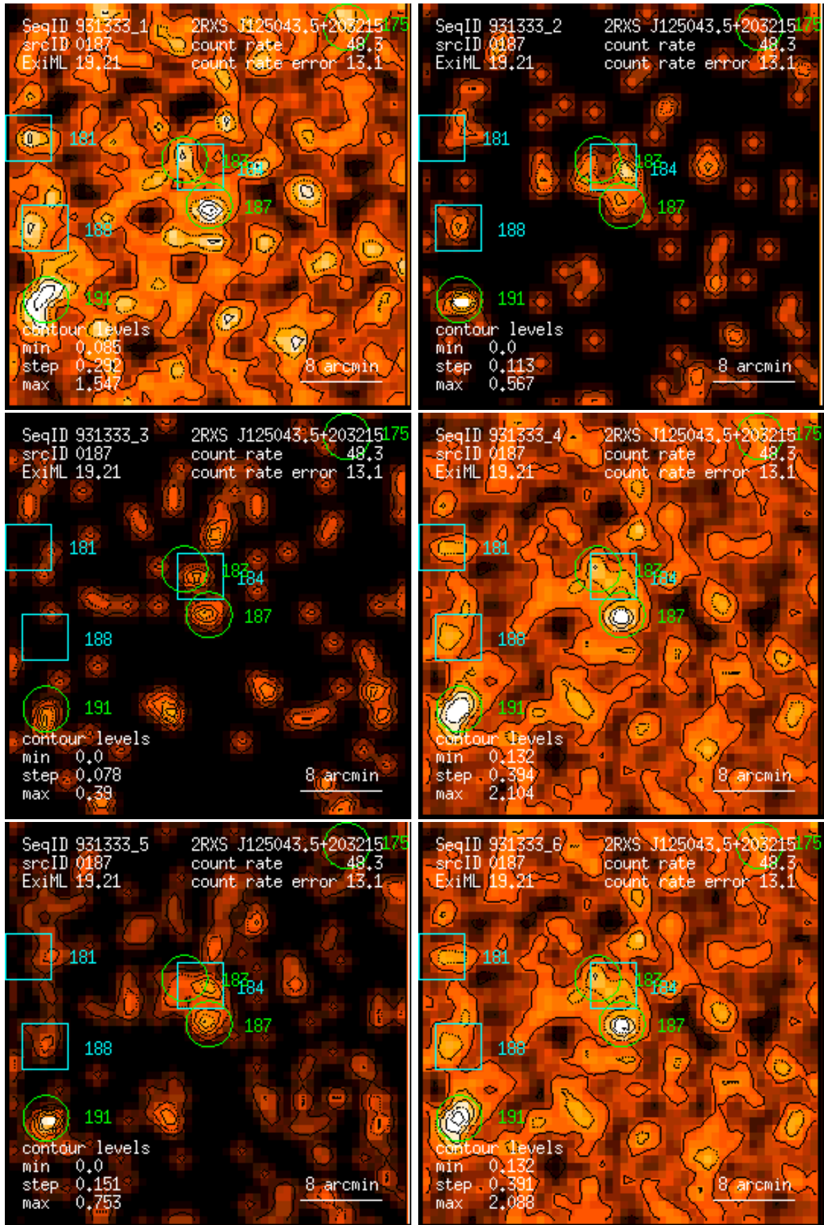
Figure 187: RASS 931333: detection 0187: band rate images, Gaussian filter: (1) PSPC channels 11 – 41, (2) 52 – 90, (3) 91 – 201, (4) 11 – 235, (5) 52 – 201, (6) 11 – 201. Broad band rates in counts/ks. Band rate contour levels in counts/ks/arcmin 2 .
