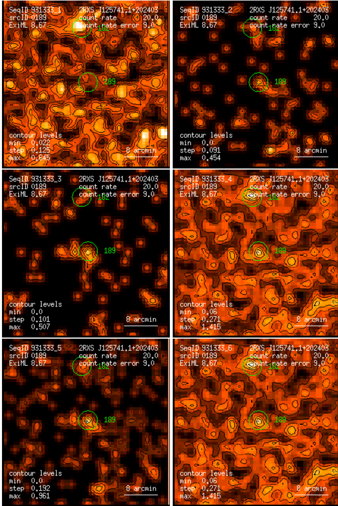
Figure 189: RASS 931333: detection 0189: band rate images, Gaussian filter: (1) PSPC channels 11 – 41, (2) 52 – 90, (3) 91 – 201, (4) 11 – 235, (5) 52 – 201, (6) 11 – 201. Broad band rates in counts/ks. Band rate contour levels in counts/ks/arcmin 2 .
