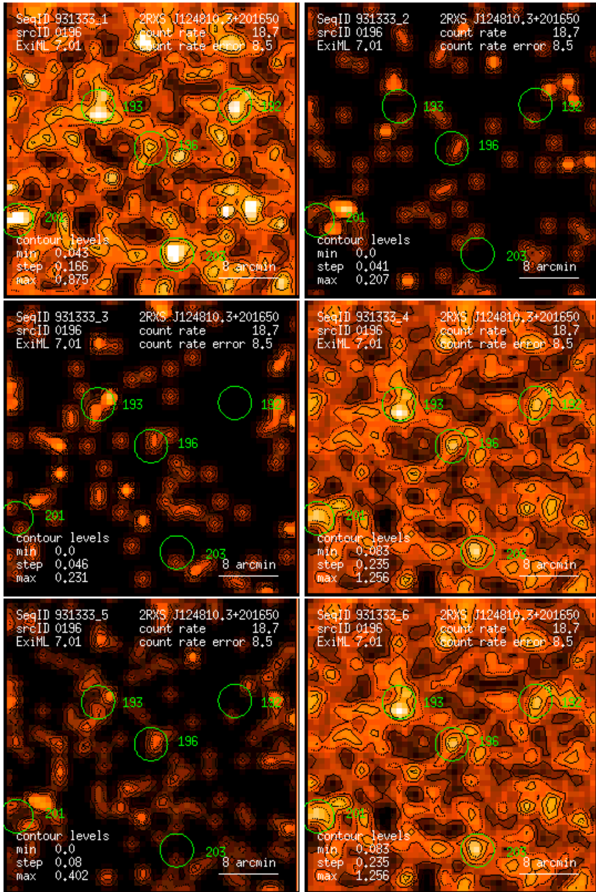
Figure 196: RASS 931333: detection 0196: band rate images, Gaussian filter: (1) PSPC channels 11 – 41, (2) 52 – 90, (3) 91 – 201, (4) 11 – 235, (5) 52 – 201, (6) 11 – 201. Broad band rates in counts/ks. Band rate contour levels in counts/ks/arcmin 2 .
