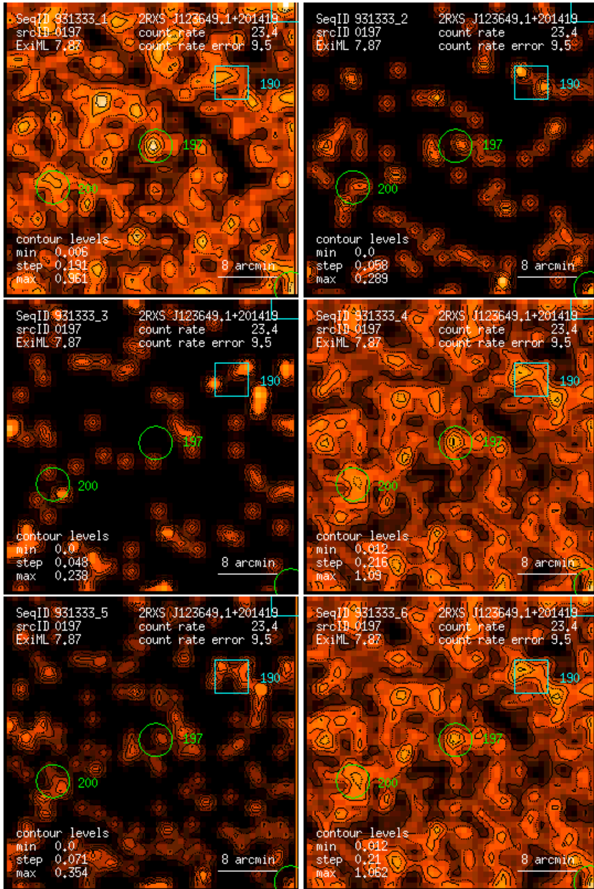
Figure 197: RASS 931333: detection 0197: band rate images, Gaussian filter: (1) PSPC channels 11 – 41, (2) 52 – 90, (3) 91 – 201, (4) 11 – 235, (5) 52 – 201, (6) 11 – 201. Broad band rates in counts/ks. Band rate contour levels in counts/ks/arcmin 2 .
