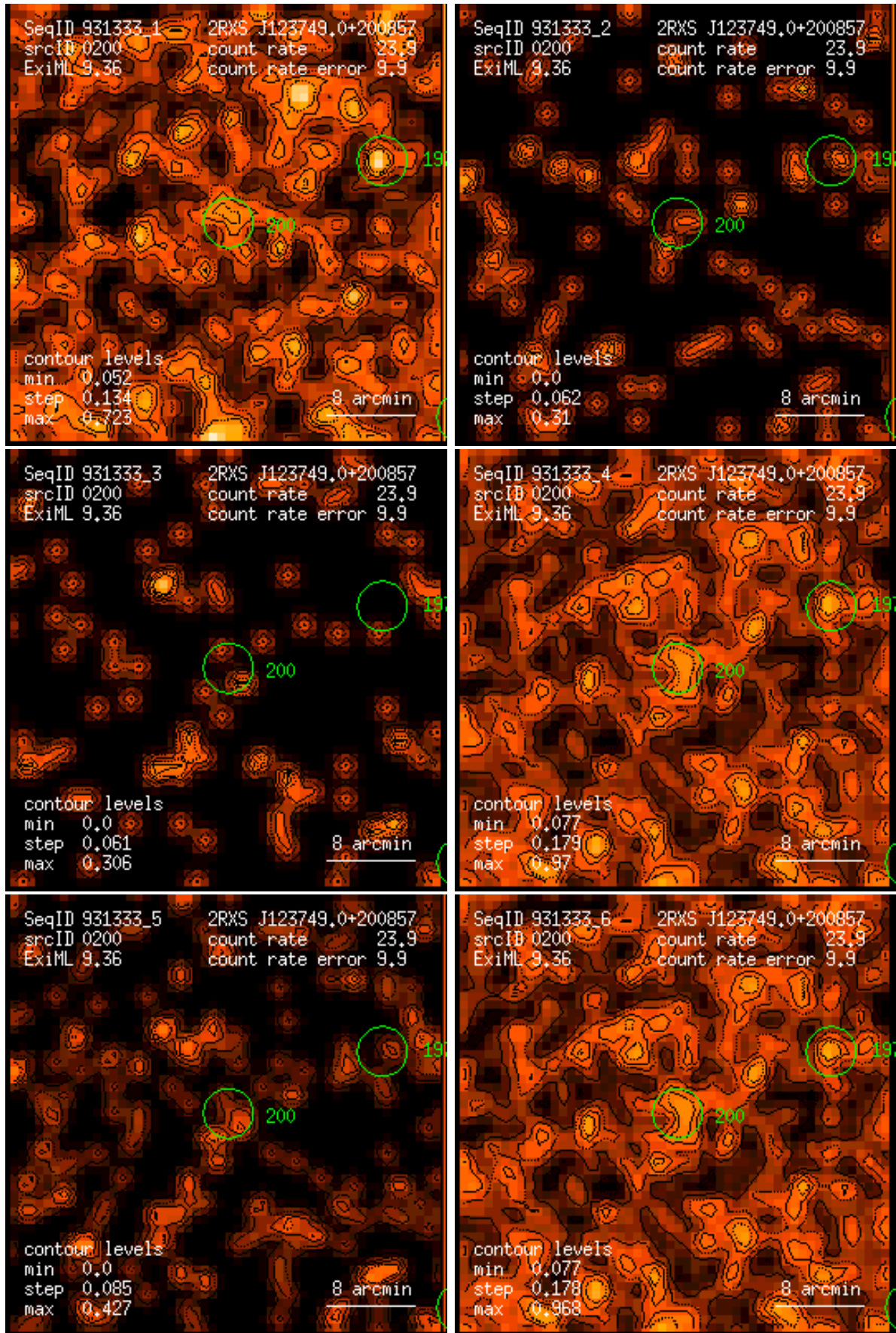
Figure 200: RASS 931333: detection 0200: band rate images, Gaussian filter: (1) PSPC channels 11 – 41, (2) 52 – 90, (3) 91 – 201, (4) 11 – 235, (5) 52 – 201, (6) 11 – 201. Broad band rates in counts/ks. Band rate contour levels in counts/ks/arcmin 2 .
