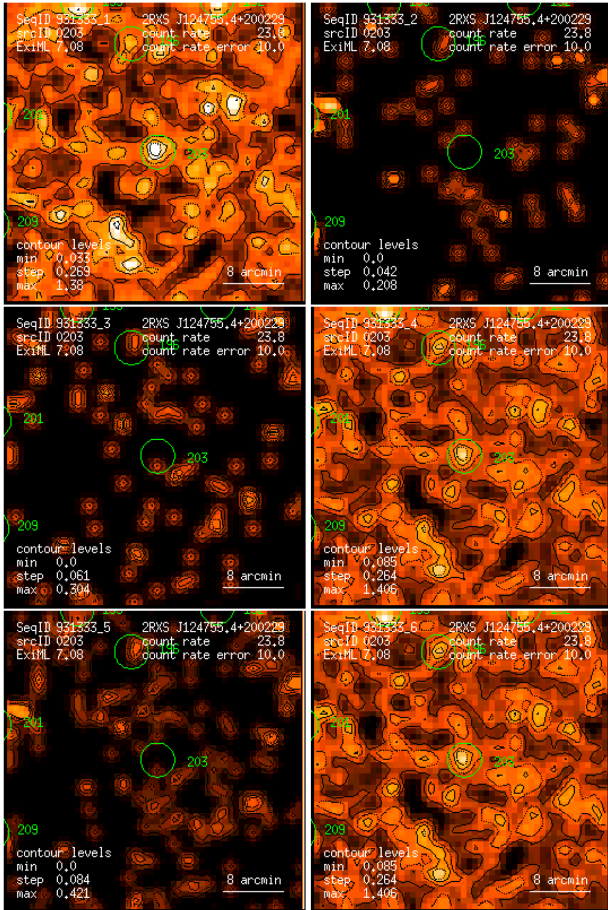
Figure 203: RASS 931333: detection 0203: band rate images, Gaussian filter: (1) PSPC channels 11 – 41, (2) 52 – 90, (3) 91 – 201, (4) 11 – 235, (5) 52 – 201, (6) 11 – 201. Broad band rates in counts/ks. Band rate contour levels in counts/ks/arcmin 2 .
