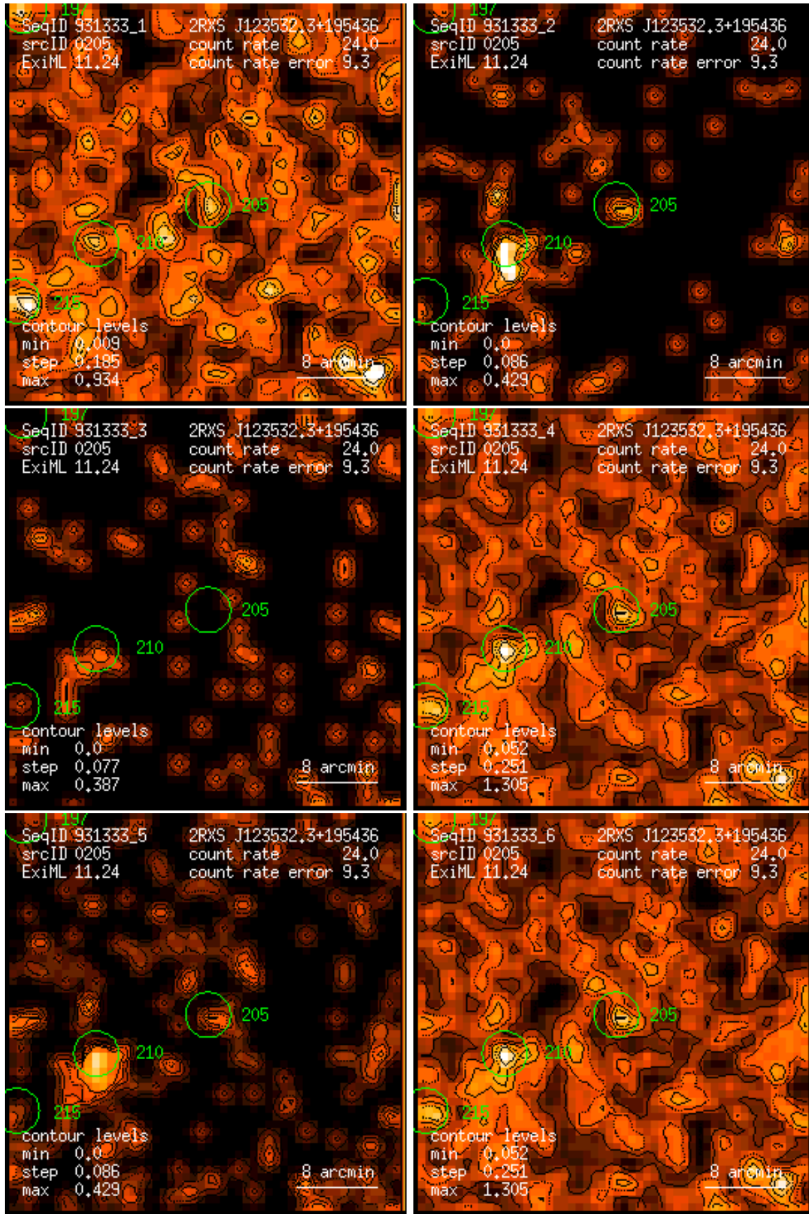
Figure 205: RASS 931333: detection 0205: band rate images, Gaussian filter: (1) PSPC channels 11 – 41, (2) 52 – 90, (3) 91 – 201, (4) 11 – 235, (5) 52 – 201, (6) 11 – 201. Broad band rates in counts/ks. Band rate contour levels in counts/ks/arcmin 2 .
