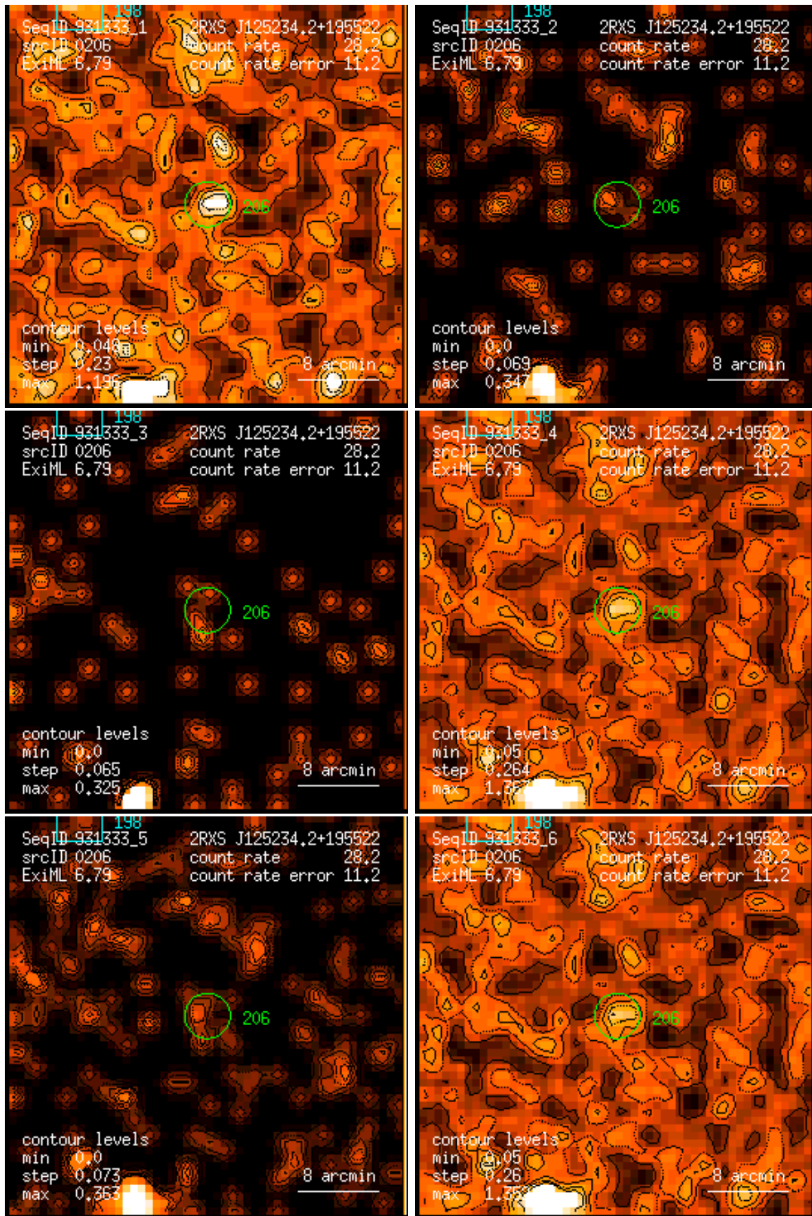
Figure 206: RASS 931333: detection 0206: band rate images, Gaussian filter: (1) PSPC channels 11 – 41, (2) 52 – 90, (3) 91 – 201, (4) 11 – 235, (5) 52 – 201, (6) 11 – 201. Broad band rates in counts/ks. Band rate contour levels in counts/ks/arcmin 2 .
