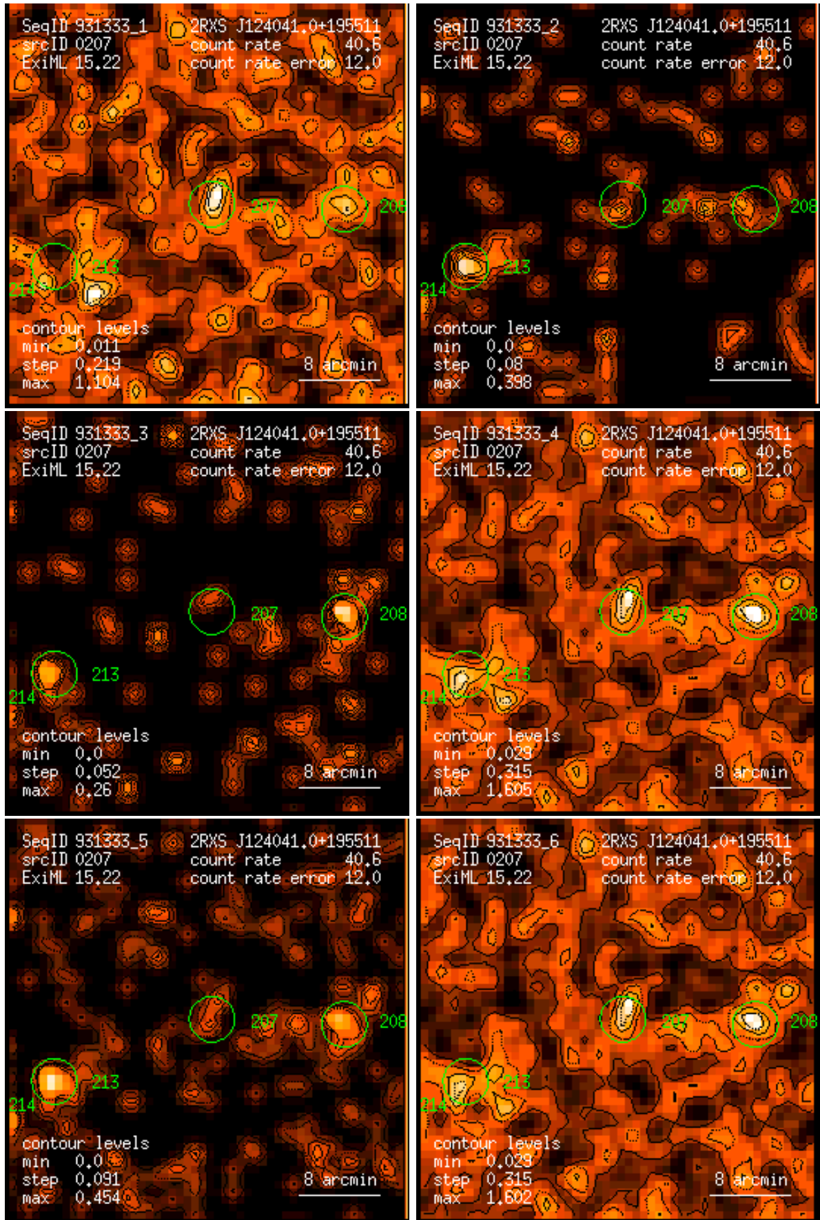
Figure 207: RASS 931333: detection 0207: band rate images, Gaussian filter: (1) PSPC channels 11 – 41, (2) 52 – 90, (3) 91 – 201, (4) 11 – 235, (5) 52 – 201, (6) 11 – 201. Broad band rates in counts/ks. Band rate contour levels in counts/ks/arcmin 2 .
