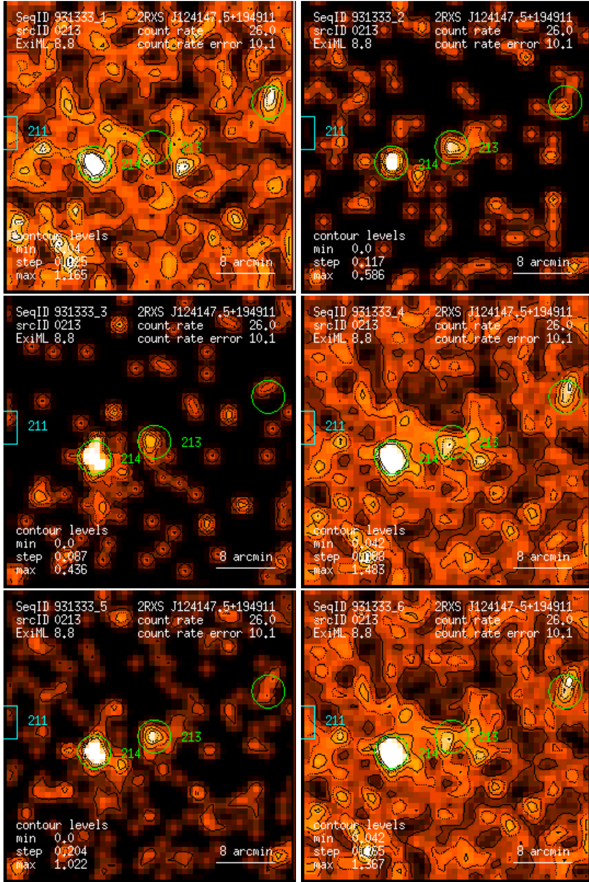
Figure 213: RASS 931333: detection 0213: band rate images, Gaussian filter: (1) PSPC channels 11 – 41, (2) 52 – 90, (3) 91 – 201, (4) 11 – 235, (5) 52 – 201, (6) 11 – 201. Broad band rates in counts/ks. Band rate contour levels in counts/ks/arcmin 2 .
