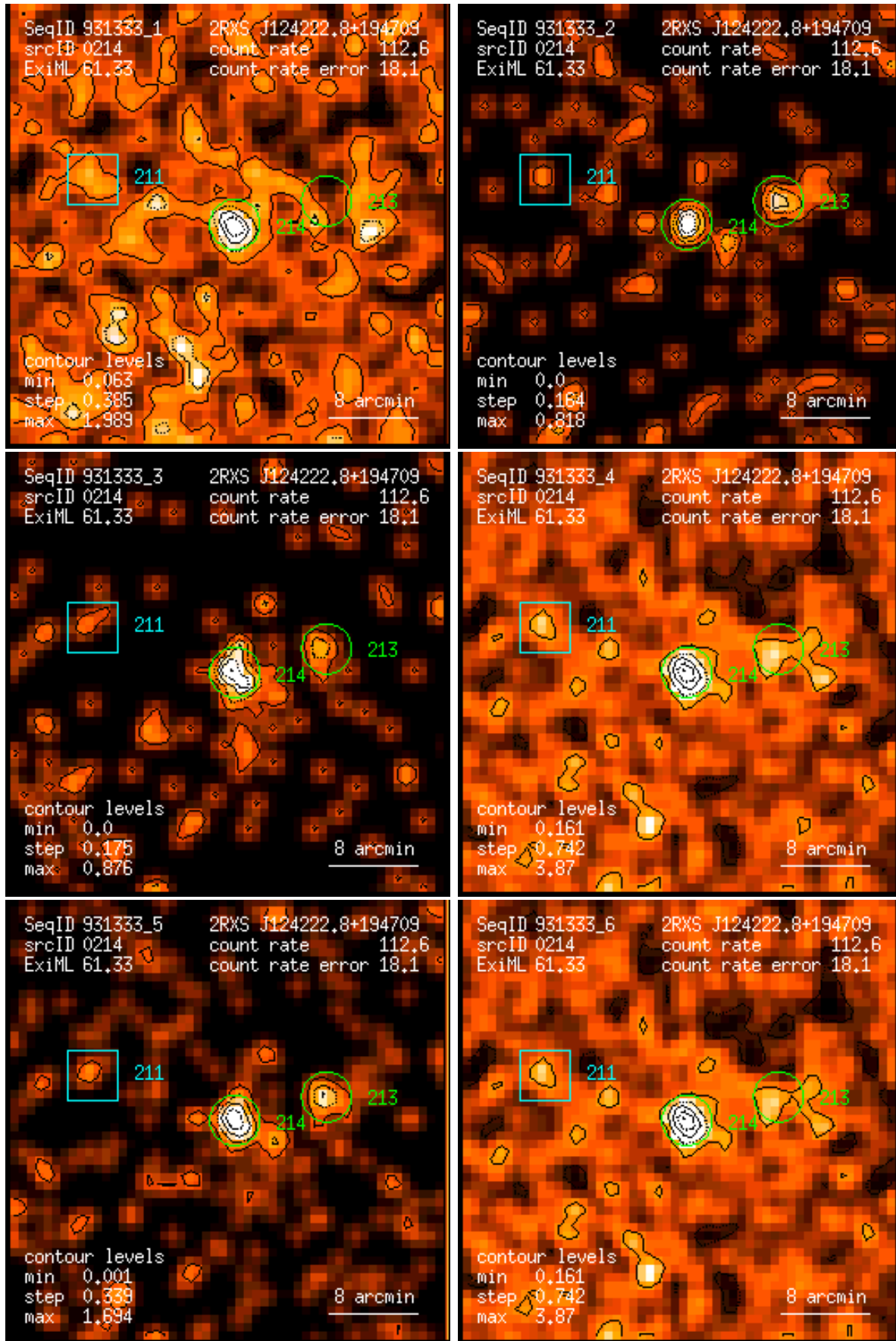
Figure 214: RASS 931333: detection 0214: band rate images, Gaussian filter: (1) PSPC channels 11 – 41, (2) 52 – 90, (3) 91 – 201, (4) 11 – 235, (5) 52 – 201, (6) 11 – 201. Broad band rates in counts/ks. Band rate contour levels in counts/ks/arcmin 2 .
