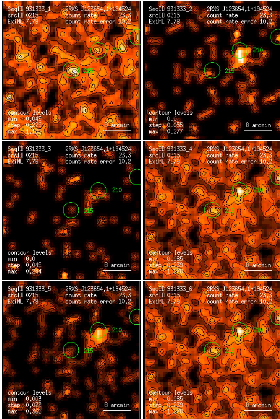
Figure 215: RASS 931333: detection 0215: band rate images, Gaussian filter: (1) PSPC channels 11 – 41, (2) 52 – 90, (3) 91 – 201, (4) 11 – 235, (5) 52 – 201, (6) 11 – 201. Broad band rates in counts/ks. Band rate contour levels in counts/ks/arcmin 2 .
