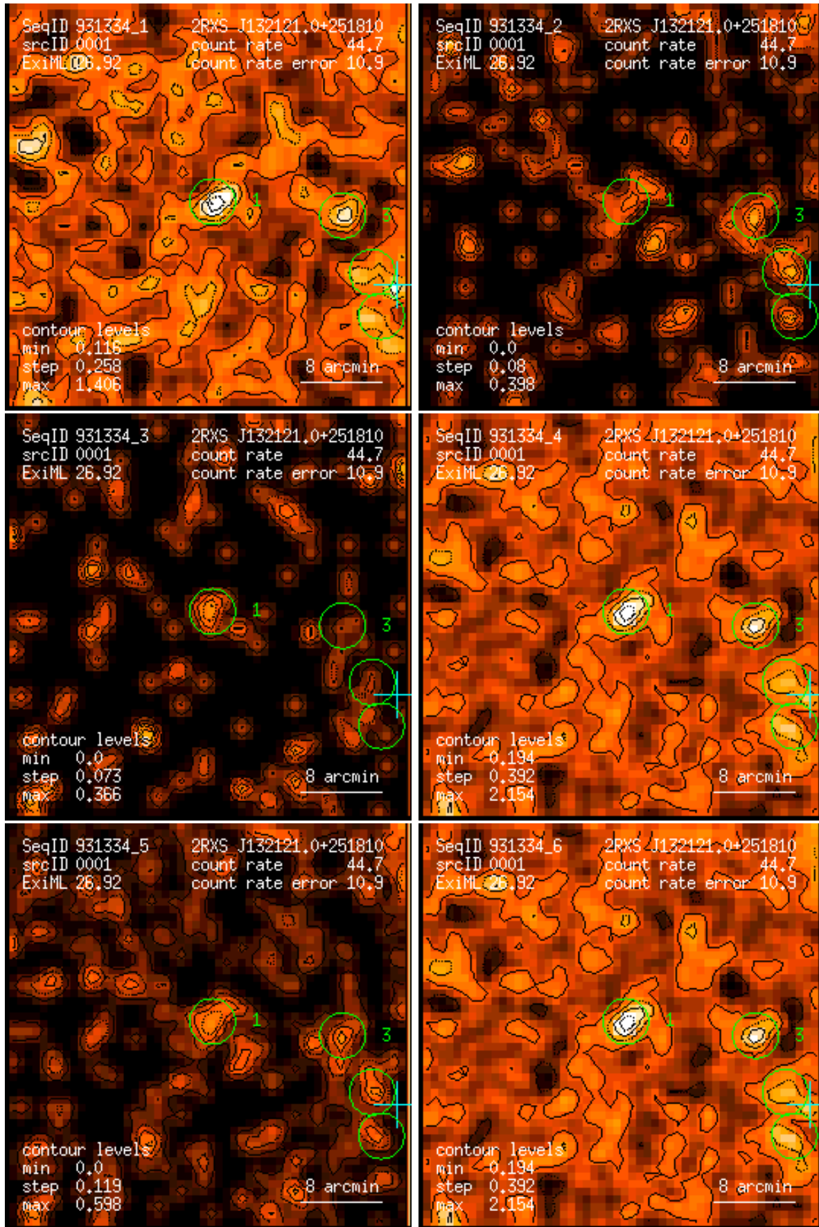
Figure 1: RASS 931334: detection 0001: band rate images, Gaussian filter: (1) PSPC channels 11 – 41, (2) 52 – 90, (3) 91 – 201, (4) 11 – 235, (5) 52 – 201, (6) 11 – 201. Broad band rates in counts/ks. Band rate contour levels in counts/ks/arcmin 2 .
