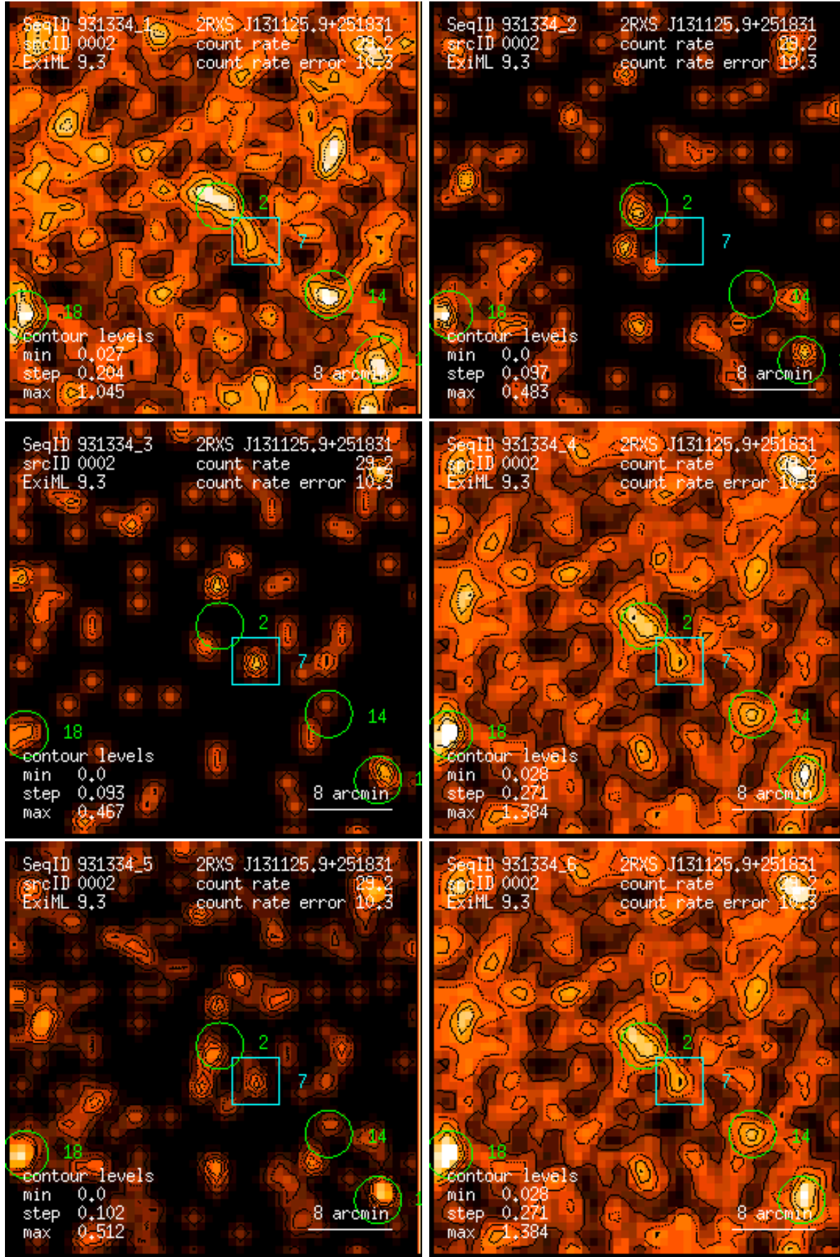
Figure 2: RASS 931334: detection 0002: band rate images, Gaussian filter: (1) PSPC channels 11 – 41, (2) 52 – 90, (3) 91 – 201, (4) 11 – 235, (5) 52 – 201, (6) 11 – 201. Broad band rates in counts/ks. Band rate contour levels in counts/ks/arcmin 2 .
