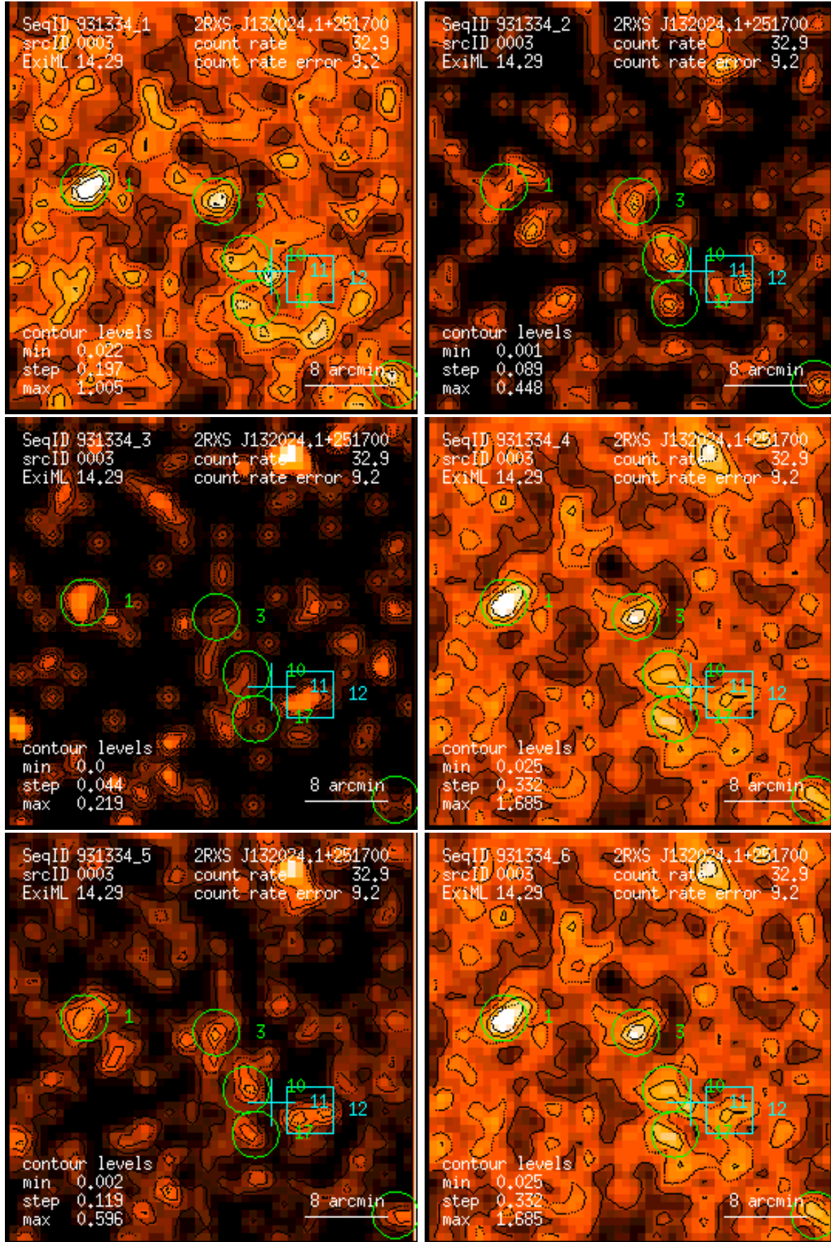
Figure 3: RASS 931334: detection 0003: band rate images, Gaussian filter: (1) PSPC channels 11 – 41, (2) 52 – 90, (3) 91 – 201, (4) 11 – 235, (5) 52 – 201, (6) 11 – 201. Broad band rates in counts/ks. Band rate contour levels in counts/ks/arcmin 2 .
