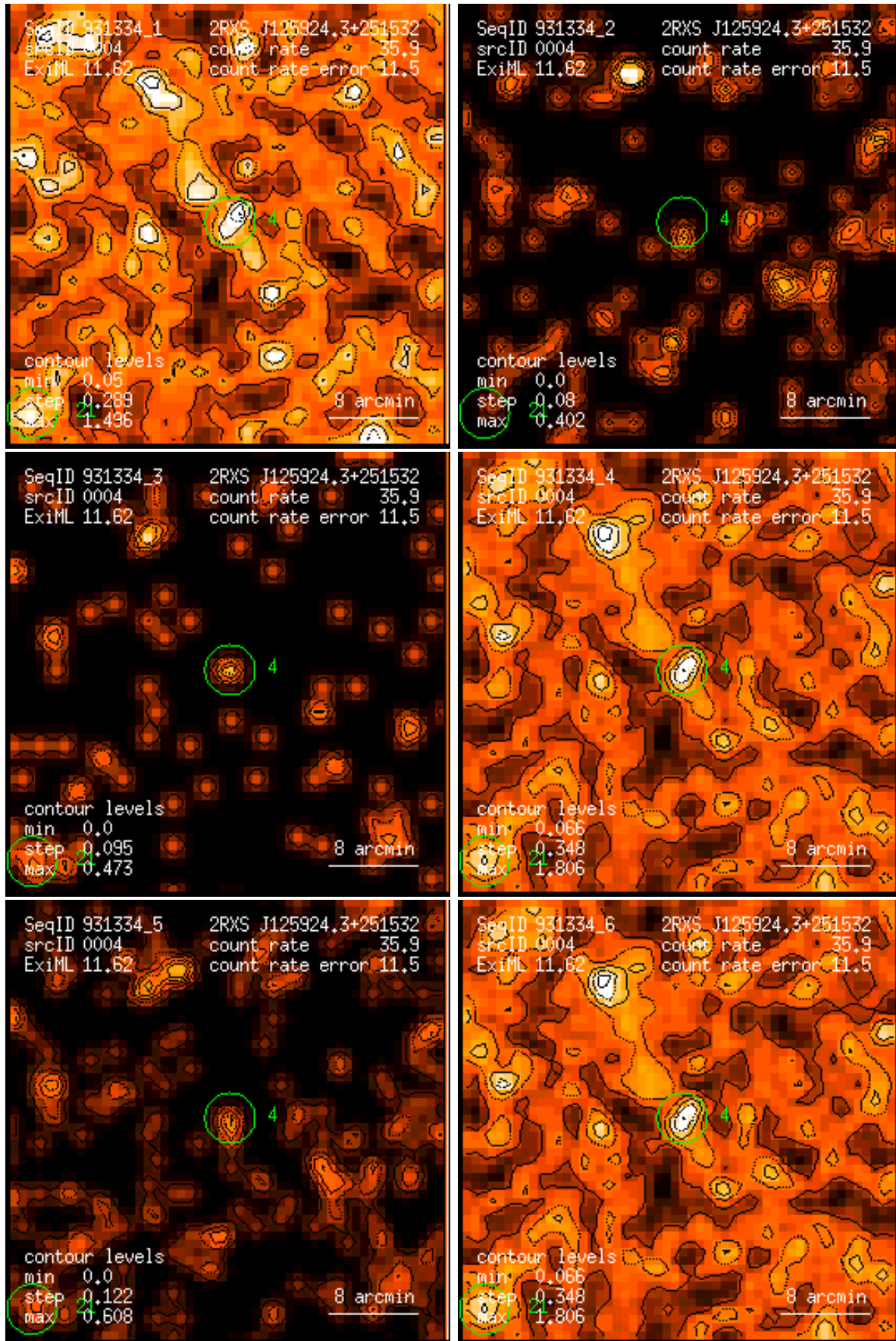
Figure 4: RASS 931334: detection 0004: band rate images, Gaussian filter: (1) PSPC channels 11 – 41, (2) 52 – 90, (3) 91 – 201, (4) 11 – 235, (5) 52 – 201, (6) 11 – 201. Broad band rates in counts/ks. Band rate contour levels in counts/ks/arcmin 2 .
