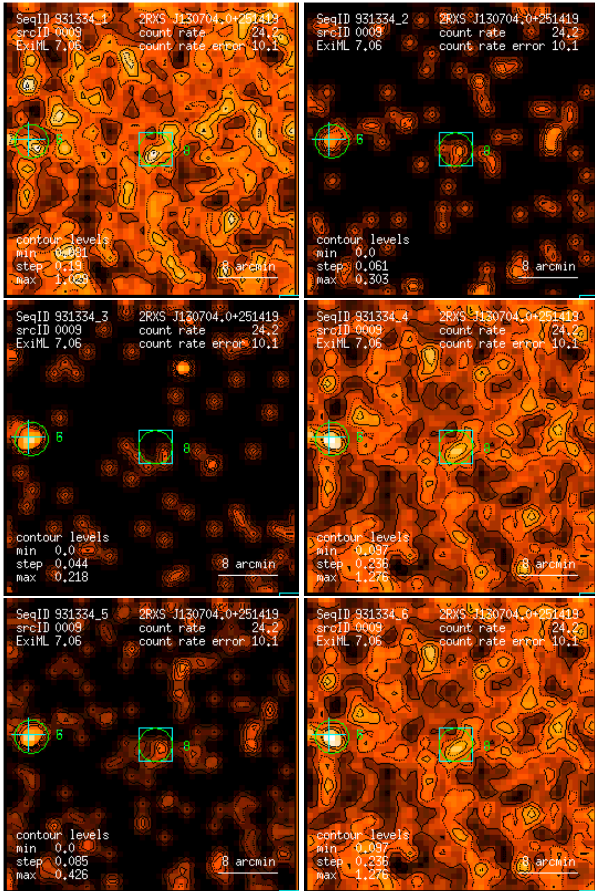
Figure 9: RASS 931334: detection 0009: band rate images, Gaussian filter: (1) PSPC channels 11 – 41, (2) 52 – 90, (3) 91 – 201, (4) 11 – 235, (5) 52 – 201, (6) 11 – 201. Broad band rates in counts/ks. Band rate contour levels in counts/ks/arcmin 2 .
