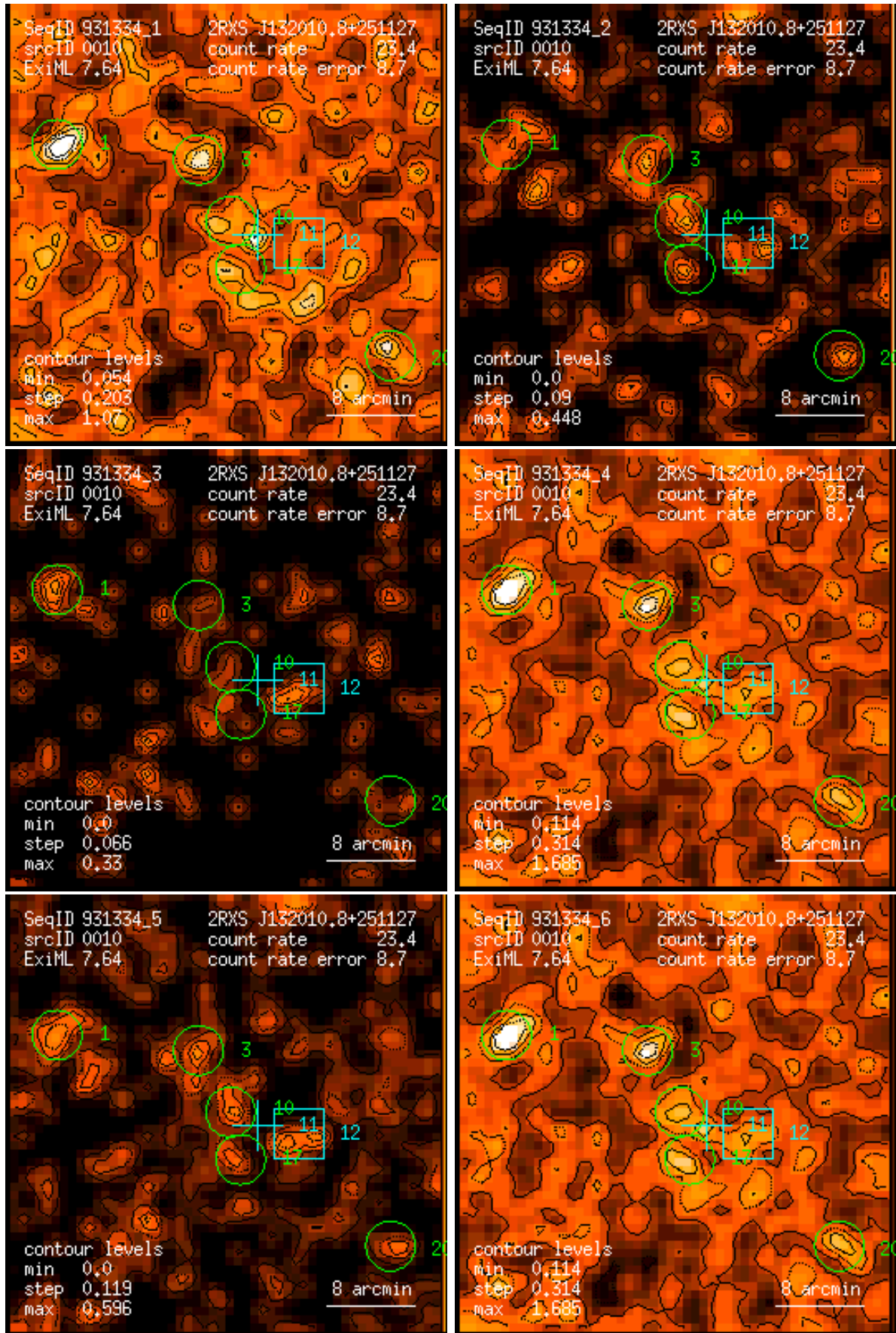
Figure 10: RASS 931334: detection 0010: band rate images, Gaussian filter: (1) PSPC channels 11 – 41, (2) 52 – 90, (3) 91 – 201, (4) 11 – 235, (5) 52 – 201, (6) 11 – 201. Broad band rates in counts/ks. Band rate contour levels in counts/ks/arcmin 2 .
