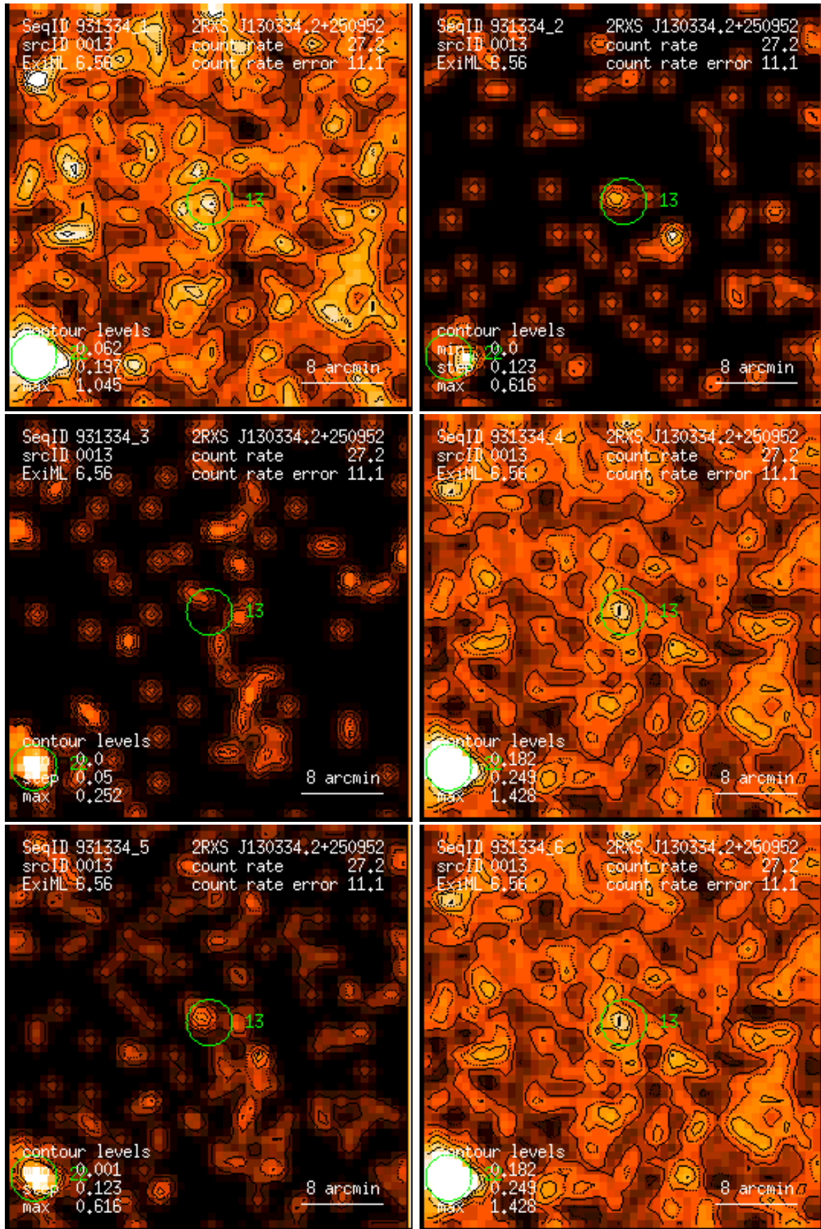
Figure 13: RASS 931334: detection 0013: band rate images, Gaussian filter: (1) PSPC channels 11 – 41, (2) 52 – 90, (3) 91 – 201, (4) 11 – 235, (5) 52 – 201, (6) 11 – 201. Broad band rates in counts/ks. Band rate contour levels in counts/ks/arcmin 2 .
