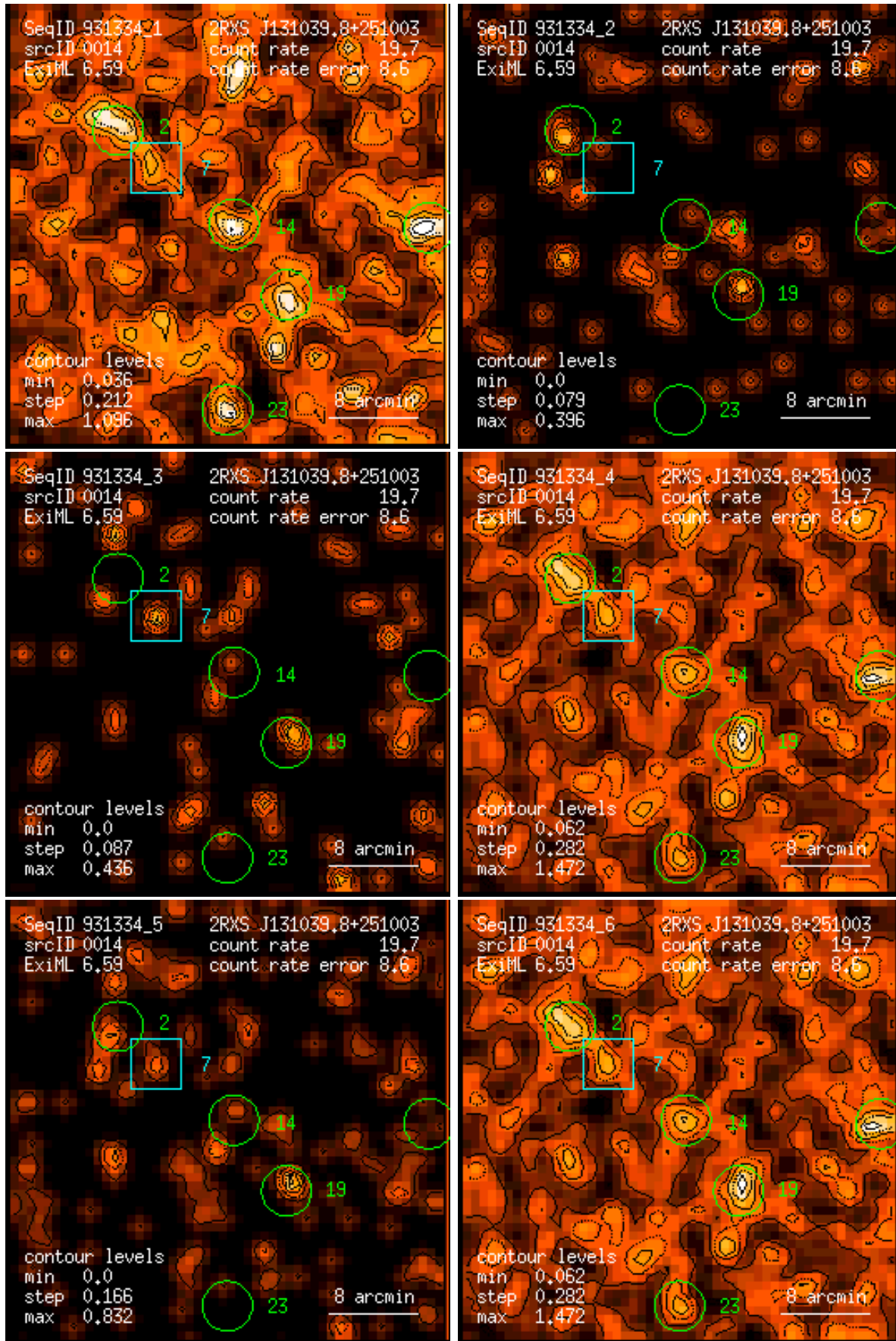
Figure 14: RASS 931334: detection 0014: band rate images, Gaussian filter: (1) PSPC channels 11 – 41, (2) 52 – 90, (3) 91 – 201, (4) 11 – 235, (5) 52 – 201, (6) 11 – 201. Broad band rates in counts/ks. Band rate contour levels in counts/ks/arcmin 2 .
