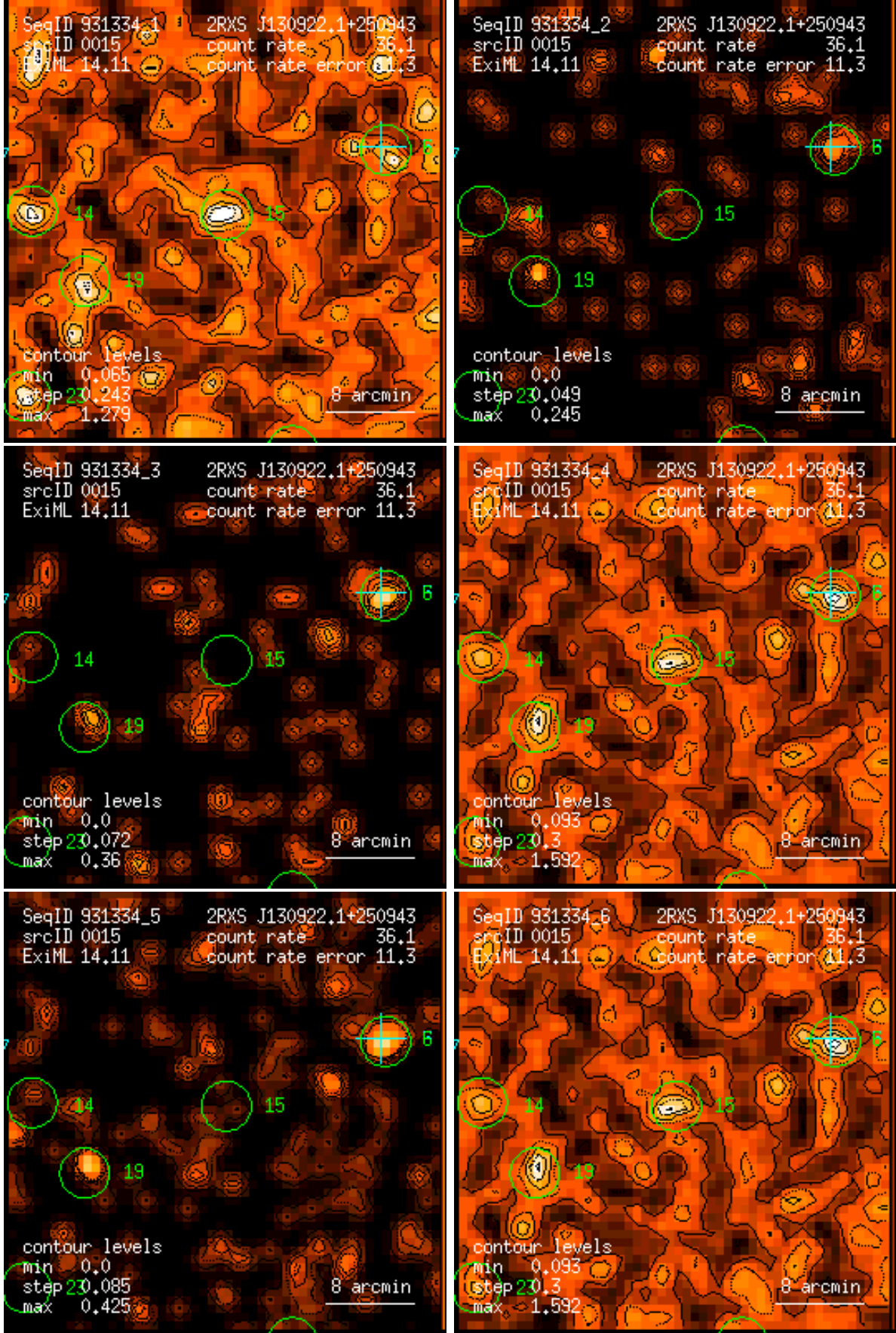
Figure 15: RASS 931334: detection 0015: band rate images, Gaussian filter: (1) PSPC channels 11 – 41, (2) 52 – 90, (3) 91 – 201, (4) 11 – 235, (5) 52 – 201, (6) 11 – 201. Broad band rates in counts/ks. Band rate contour levels in counts/ks/arcmin 2 .
