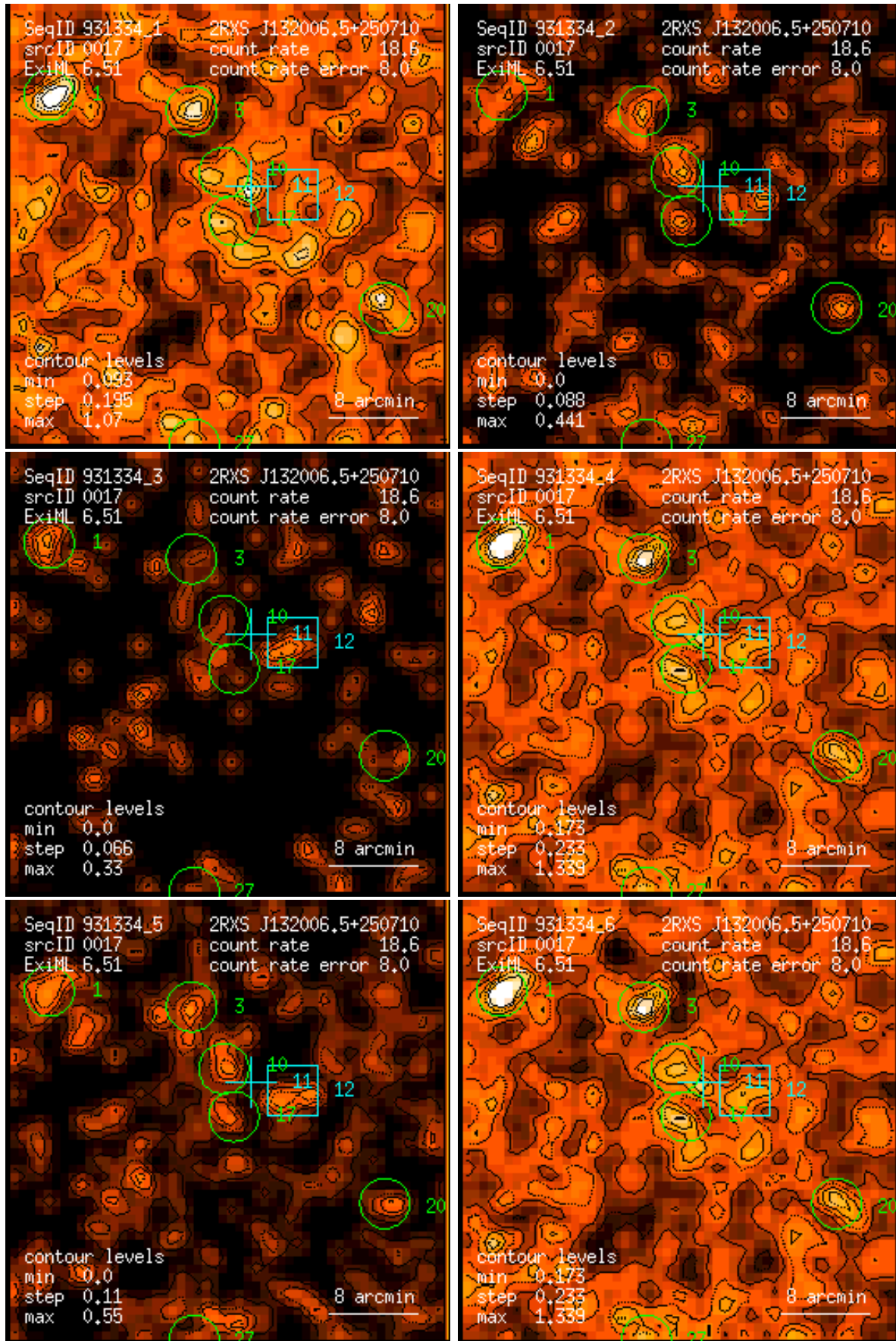
Figure 17: RASS 931334: detection 0017: band rate images, Gaussian filter: (1) PSPC channels 11 – 41, (2) 52 – 90, (3) 91 – 201, (4) 11 – 235, (5) 52 – 201, (6) 11 – 201. Broad band rates in counts/ks. Band rate contour levels in counts/ks/arcmin 2 .
