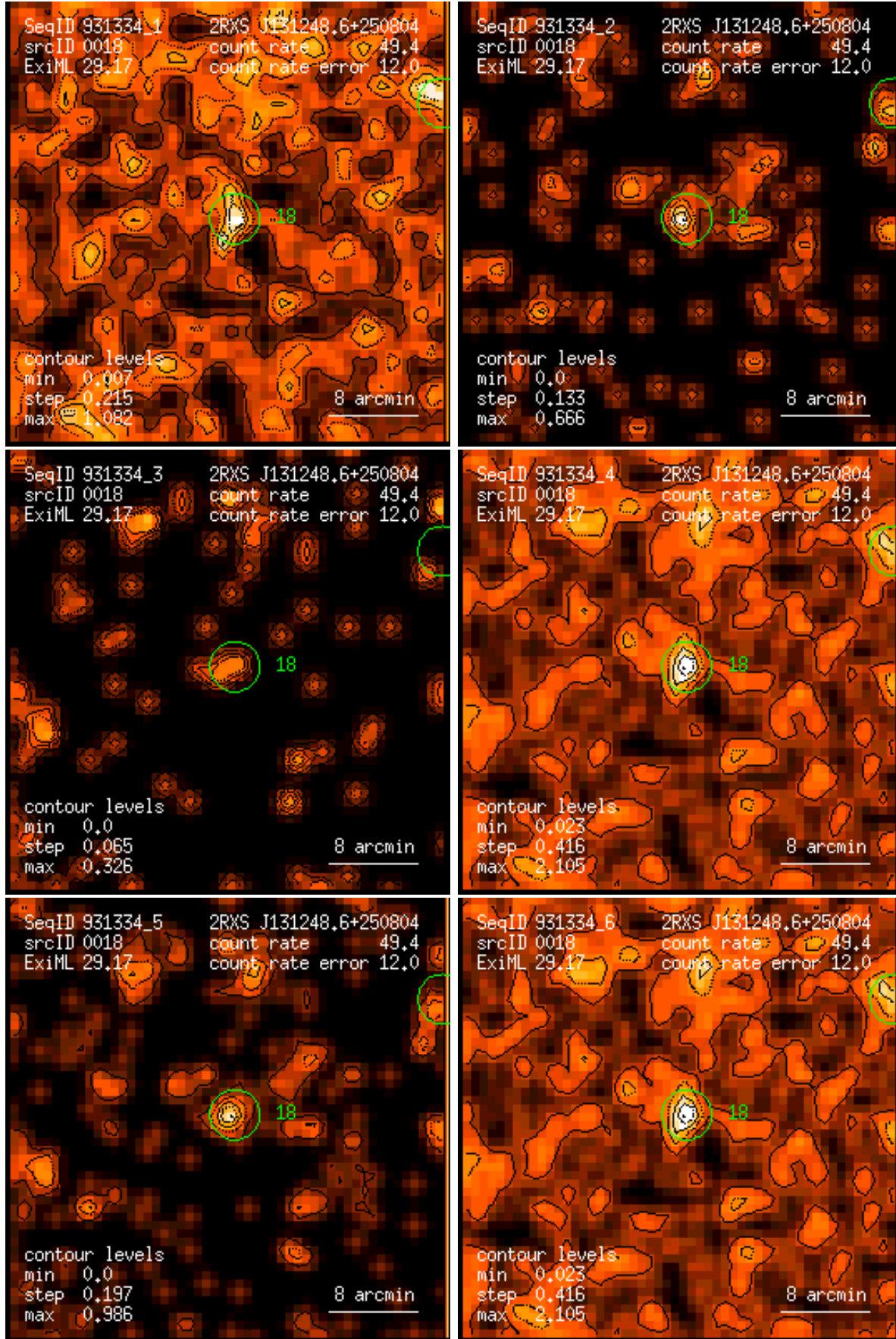
Figure 18: RASS 931334: detection 0018: band rate images, Gaussian filter: (1) PSPC channels 11 – 41, (2) 52 – 90, (3) 91 – 201, (4) 11 – 235, (5) 52 – 201, (6) 11 – 201. Broad band rates in counts/ks. Band rate contour levels in counts/ks/arcmin 2 .
